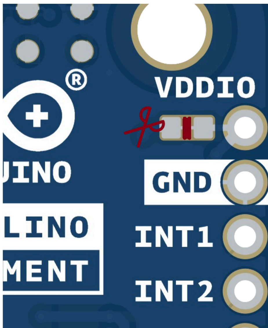
Optional jumper
