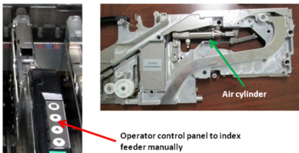
Figure 16. Examples of an electric feeder (left) and a pneumatic feeder (right), which are typically used in pick and place machines to advance the tape with LEDs.
