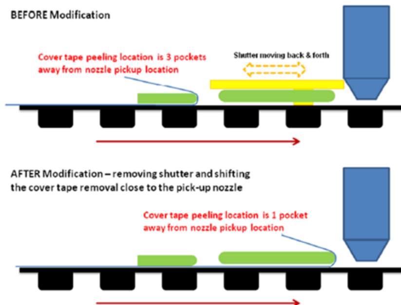
Figure 18. Illustration of the general principle behind the feeder modification.
