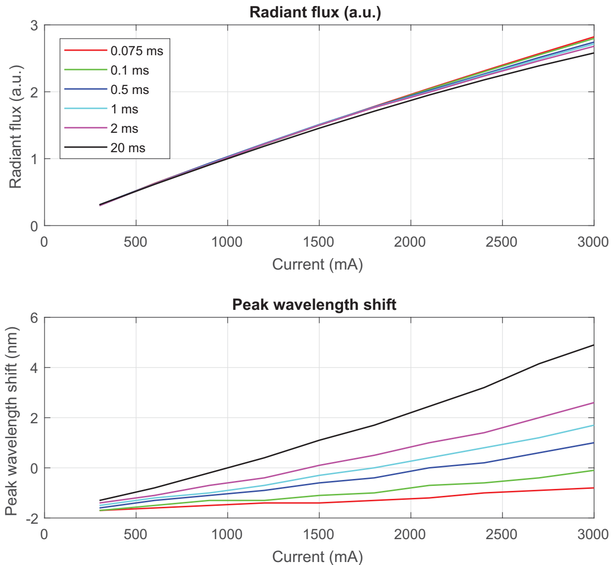
Figure 7. Typical behavior of output flux and peak wavelength shift at different forward currents, and pulse lengths for 850 nm LUXEON IR Family products. Plot color indicates pulse length. Case temperature T_c = 25^\circ\text{C} .
