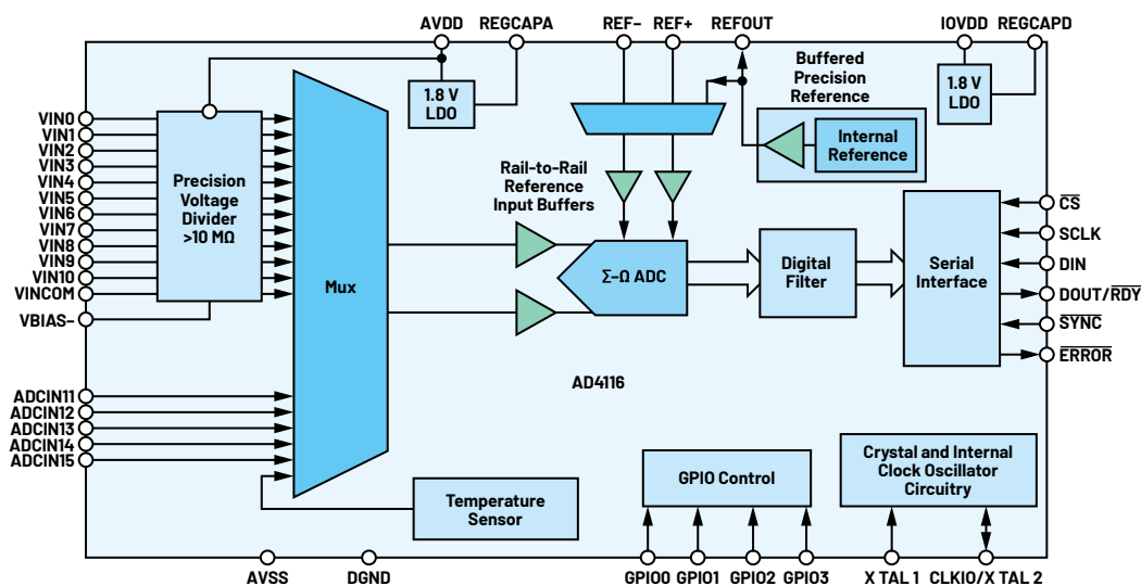
Figure 1. The internal structure of a new-generation multiplexed ADC.
