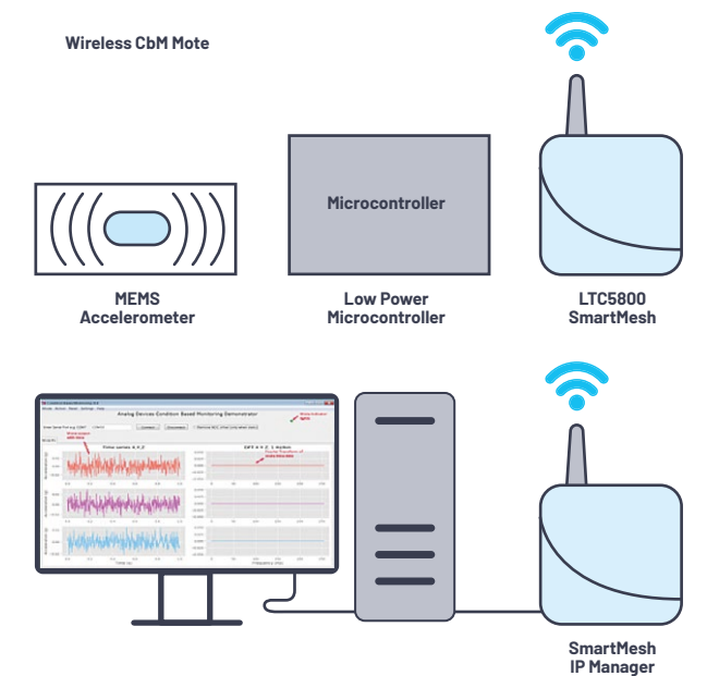
Figure 8. High level overview of Voyager hardware and GUI.
