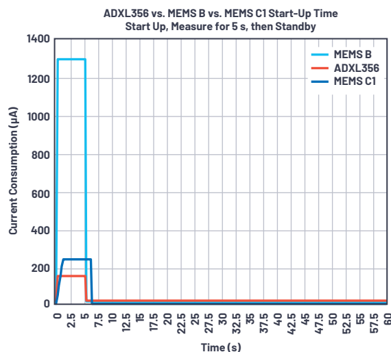
Figure 16. Current consumption for the ADXL356, MEMS B, and MEMS C1 for startup, then a 5 s measurement at the worst-case start-up time for MEMS C1 over 60 s.
