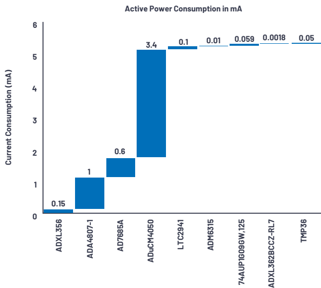
Figure 11. Signal chain power consumption in active mode.
