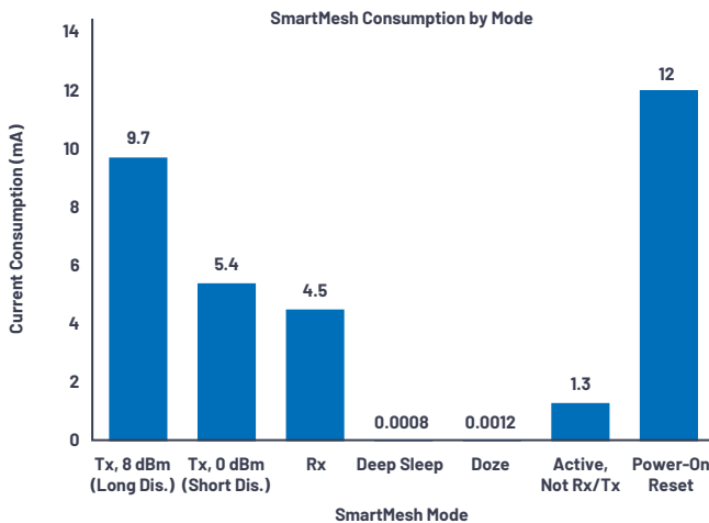
Figure 18. SmartMesh IP current consumption (worst-case data sheet specifications).
