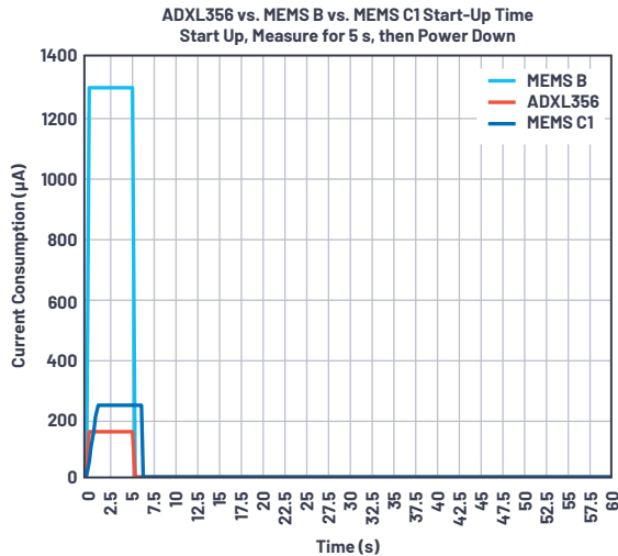
Figure 17. Current consumption for the ADXL356, MEMS B, and MEMS C1 for startup, then a 5 s measurement, then powering down over 60 s.
