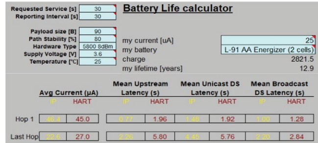
Figure 19. The SmartMesh Power and Performance Estimator tool.
