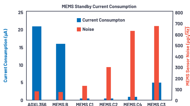
Figure 14. Comparison of MEMS sensor active current consumption vs. noise density.
