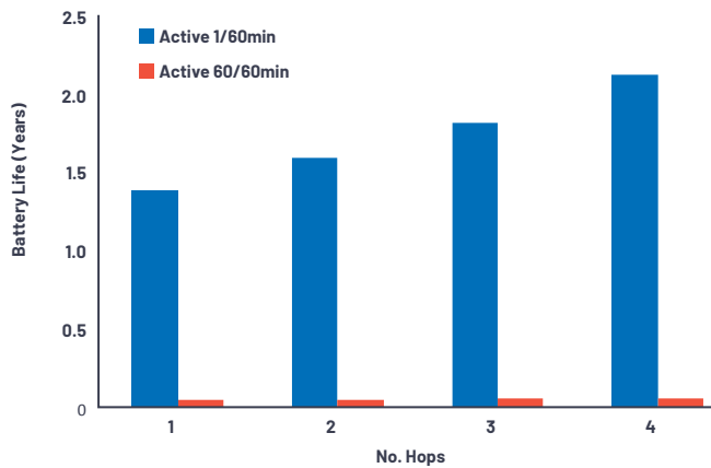
Figure 21. SmartMesh battery life vs. the number of required hops to transmit data.
