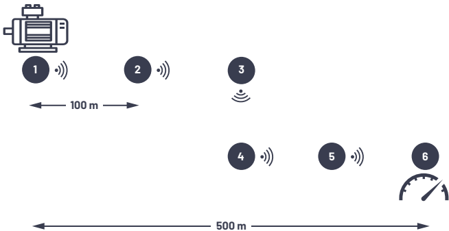
Figure 2. A mesh network implemented on the factory floor showing data hopping.
