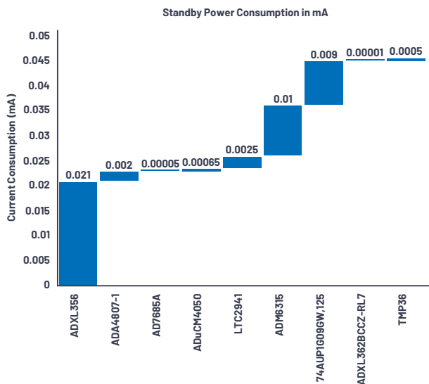
Figure 12. Signal chain power consumption in standby mode.
