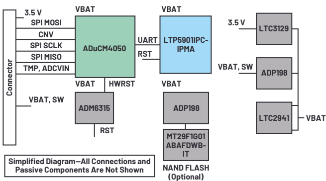
Figure 10. A high level block diagram of the ADuCM4050/SmartMesh.
