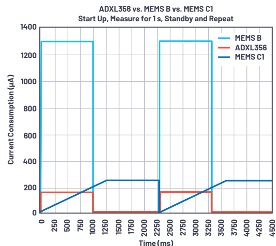
Figure 15. Current consumption for the ADXL356, MEMS B, and MEMS C1 for startup, then a 1 s measurement at the worst-case start-up time for MEMS C1 repeated twice over 4.5 s.
