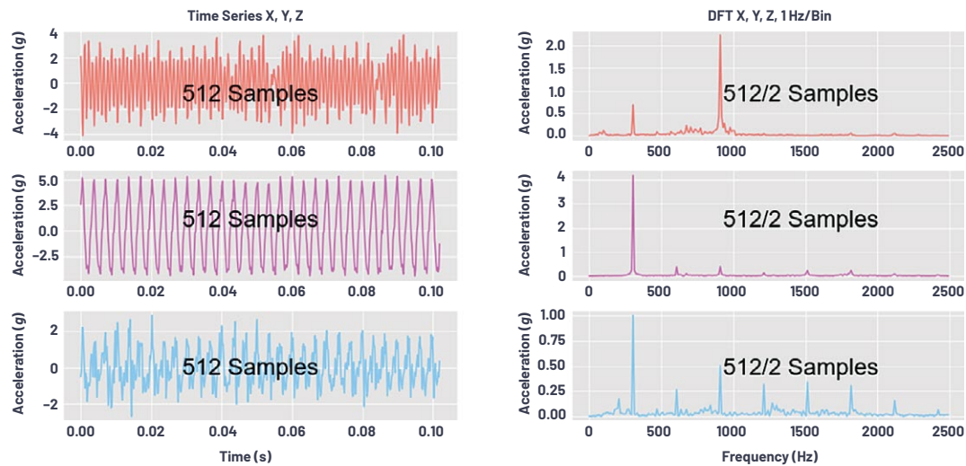
Figure 20. A Voyager GUI showing time domain and frequency domain data.
