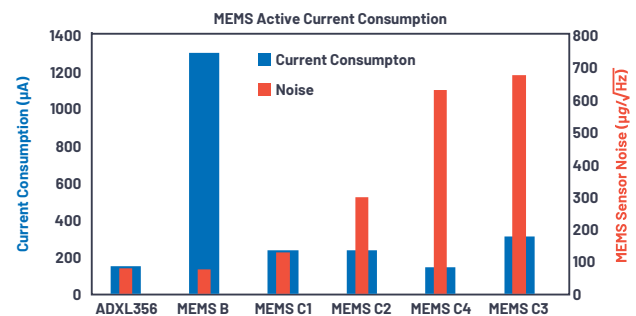
Figure 13. Comparison of MEMS sensor standby current consumption vs. noise density.
