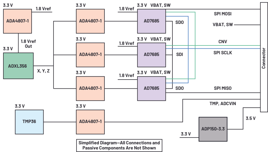
Figure 9. A high level block diagram of the ADXL356 signal chain.
