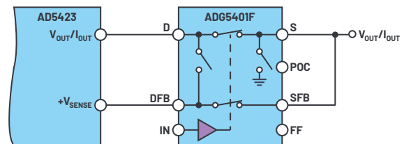
Figure 1. AD5423 and ADG5401F configuration.
