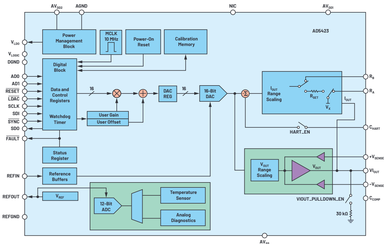
Figure 3. AD5423 functional block diagram.
