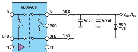
Figure 2. ADG5401F circuit diagram.
