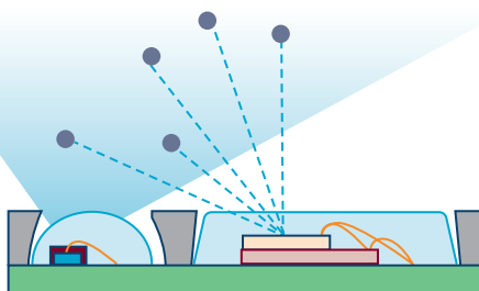
Figure 4. Schematic of the ADPD188BI.
