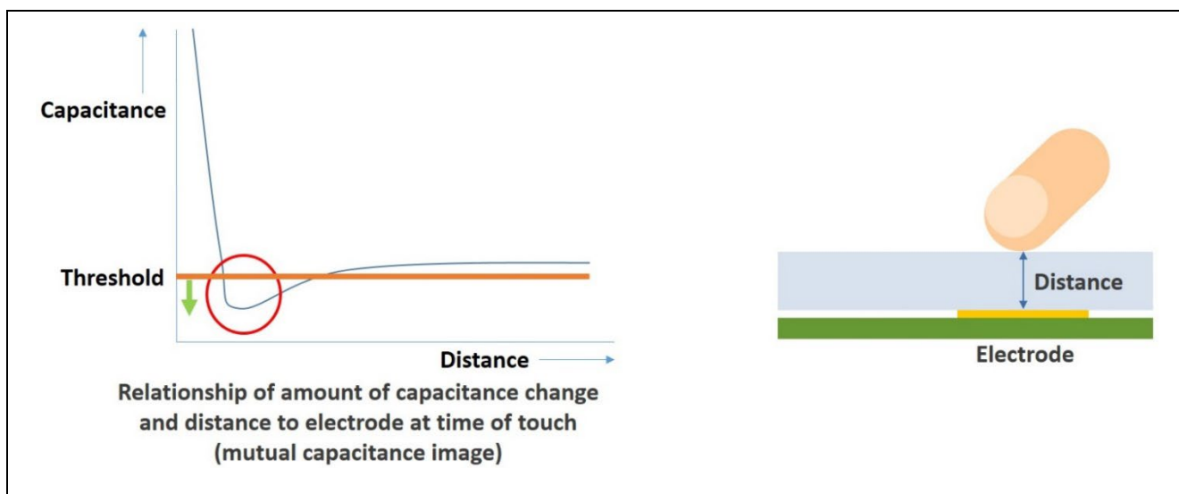
Figure3-9. Relationship of Capacitance Change and Sensitivity Distance for Mutual-capacitance Method
