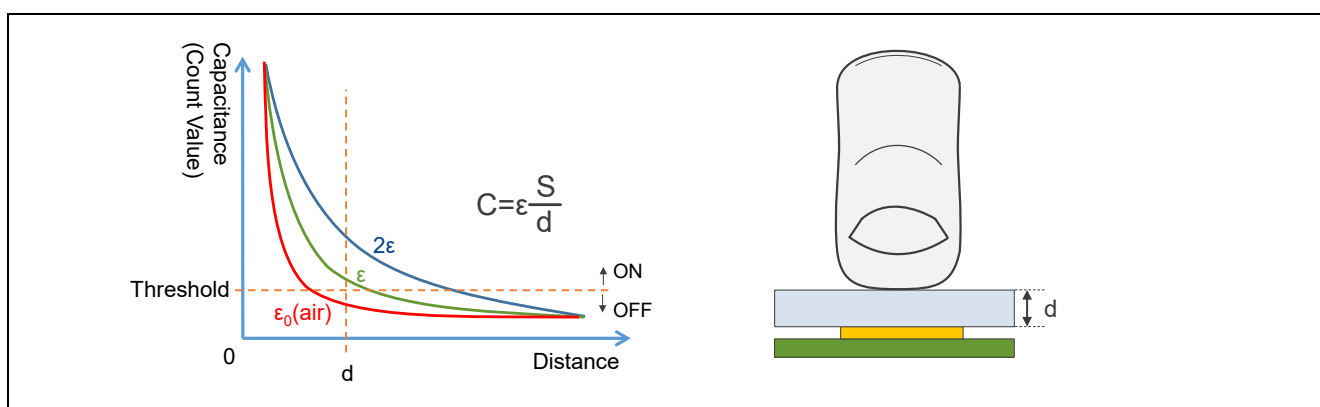
Figure2-20. Relationship of Capacitance Change and Sensitivity Distance
