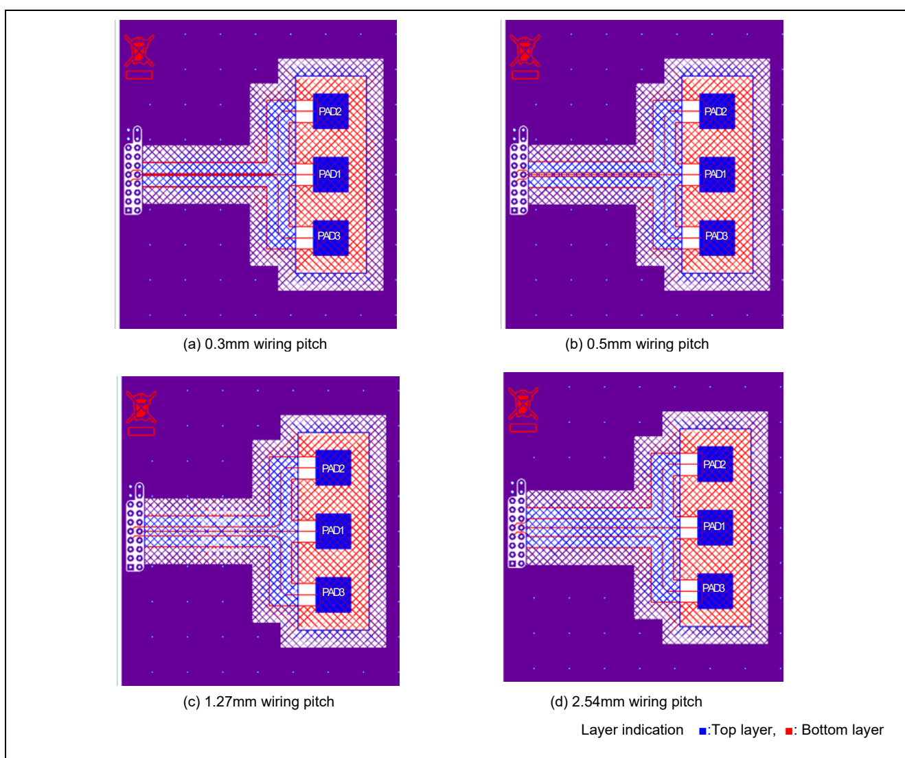
Figure 5-13 Evaluation Board Pattern (wiring length = 50mm)
