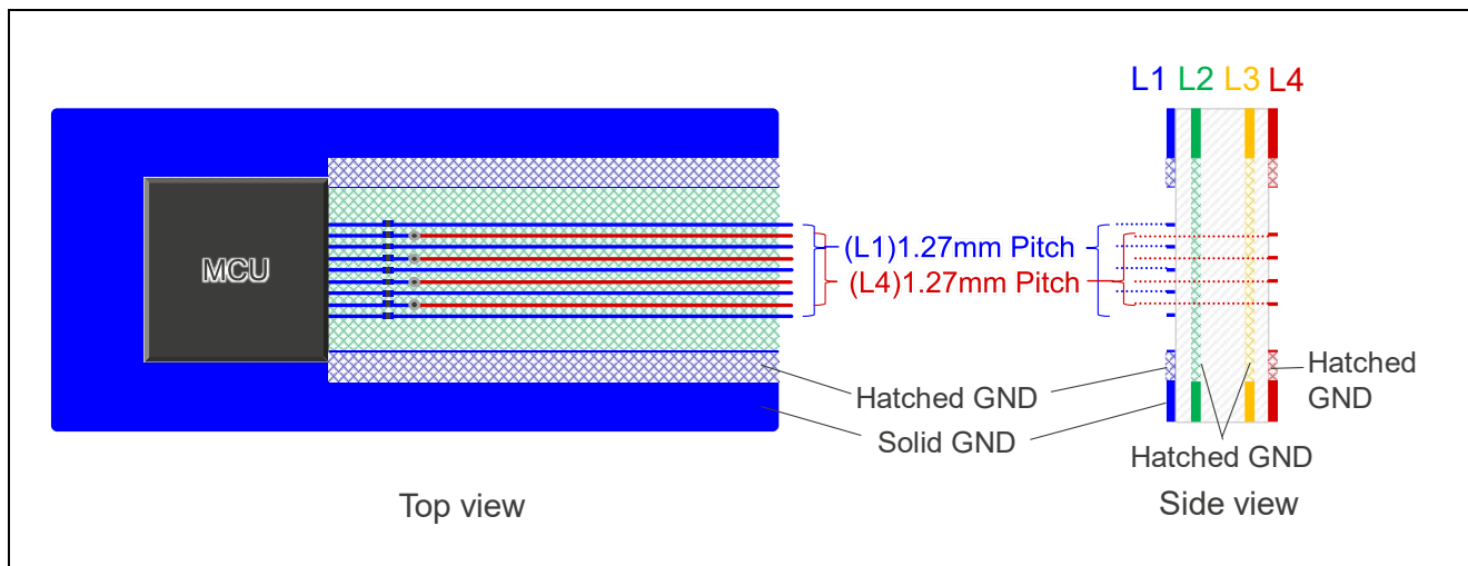
Figure2-13. High-density Wiring
