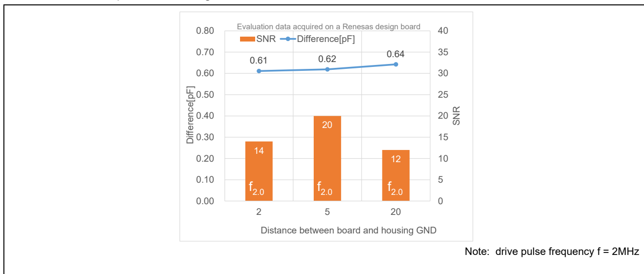
Figure 5-56 Board-Housing GND Distance and Sensitivity Characteristics
