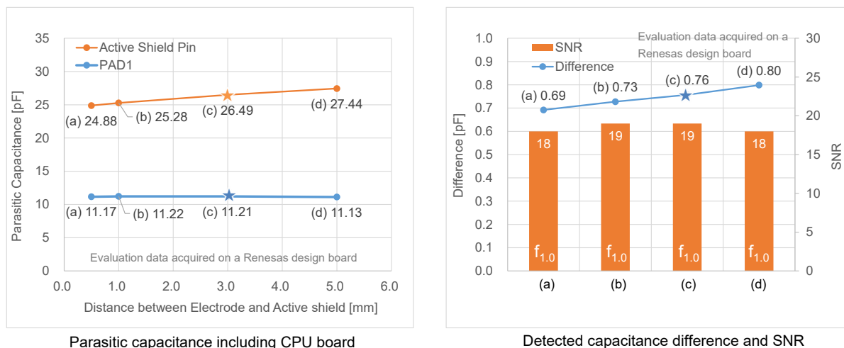
Figure 5-39 Electrode-Active Shield Distance and Sensitivity Characteristics
