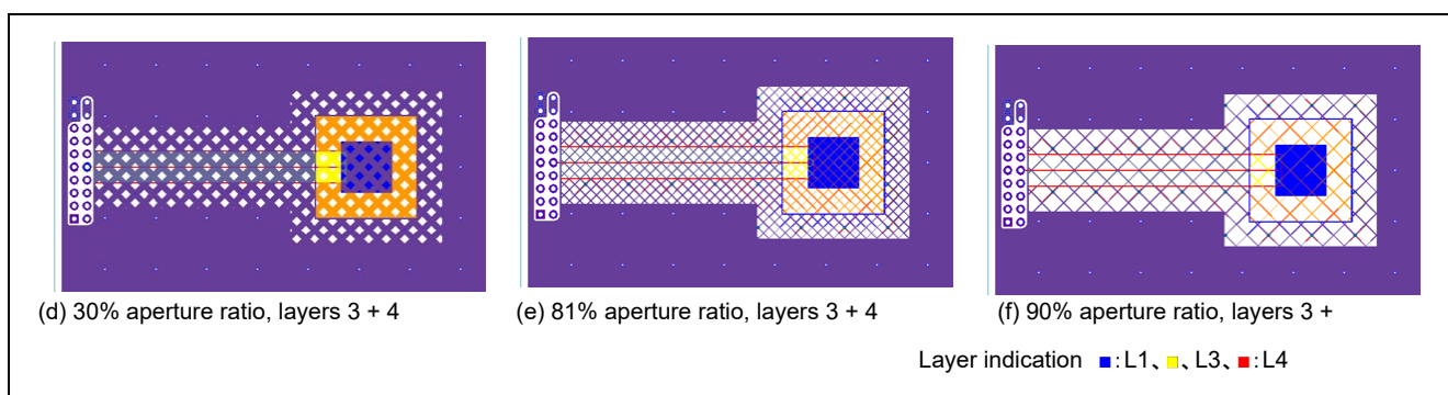
Figure 5-34 Evaluation Board Patterns (4-layered board, GND shield)
