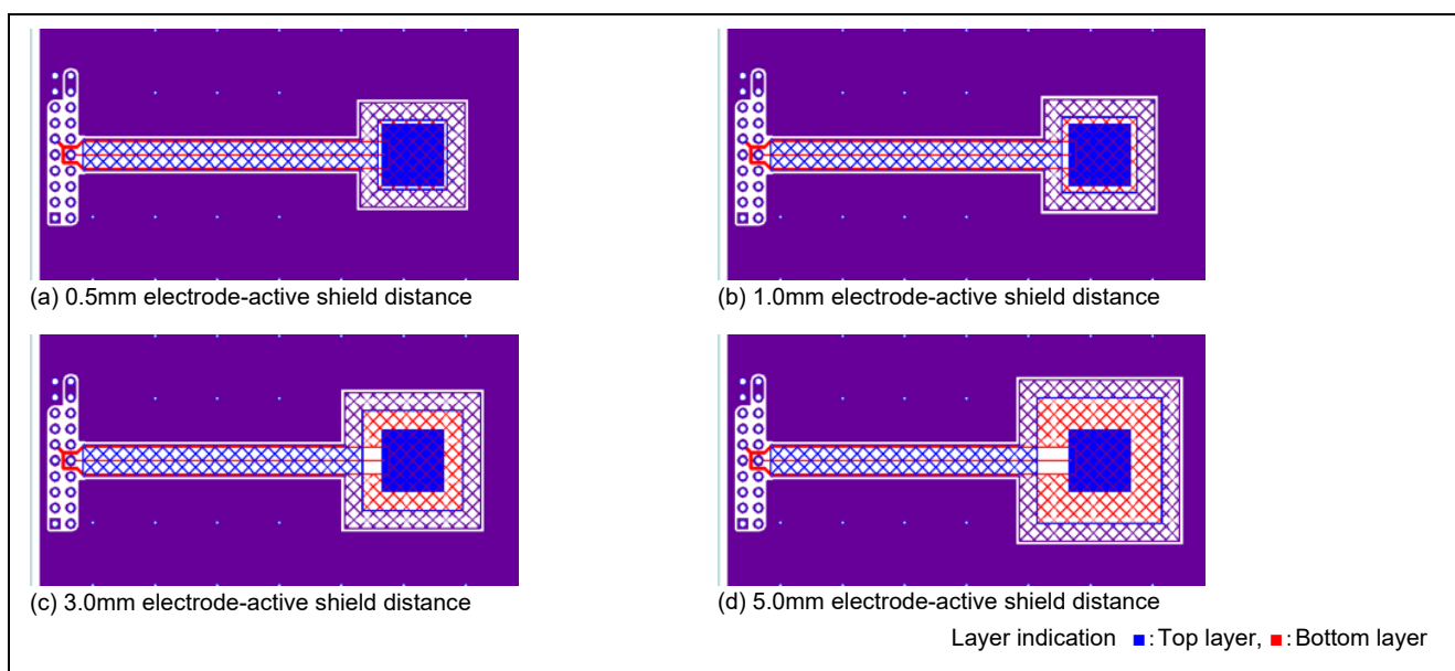
Figure 5-38 Evaluation Board Pattern
