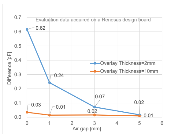
Figure 5-51 Overlay Air Gap and Parasitic Capacitance
