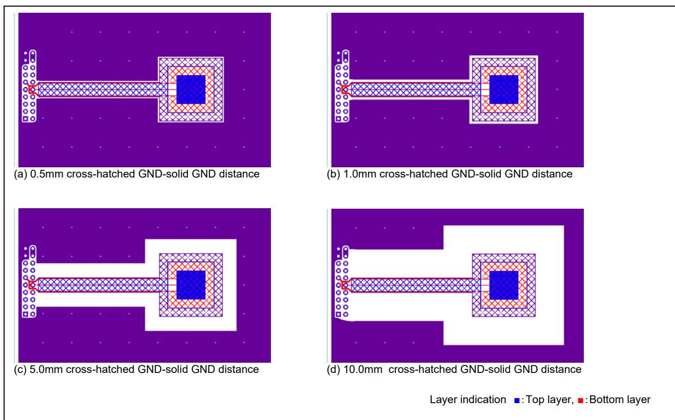
Figure 5-42 Evaluation Board Pattern (active shield-solid GND distance and sensitivity characteristics)
