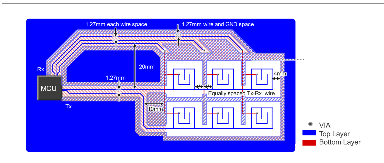
Figure3-11. Example of Electrode Routing for Mutual-capacitance Method
