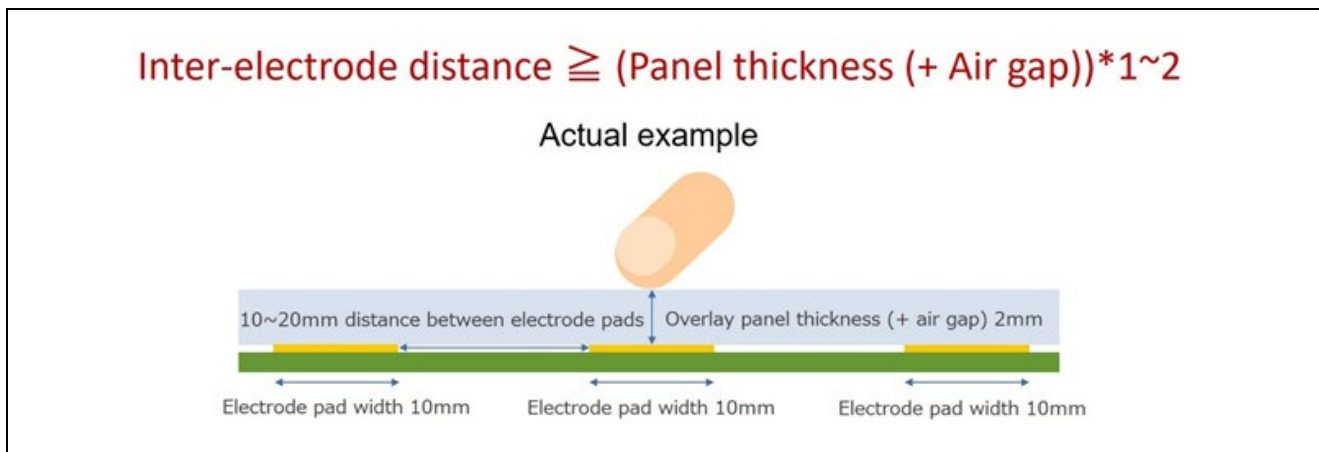
Figure3-18. Relationship of Water-resistant Inter-electrode Distance and Overlay for Mutual-capacitance Method
