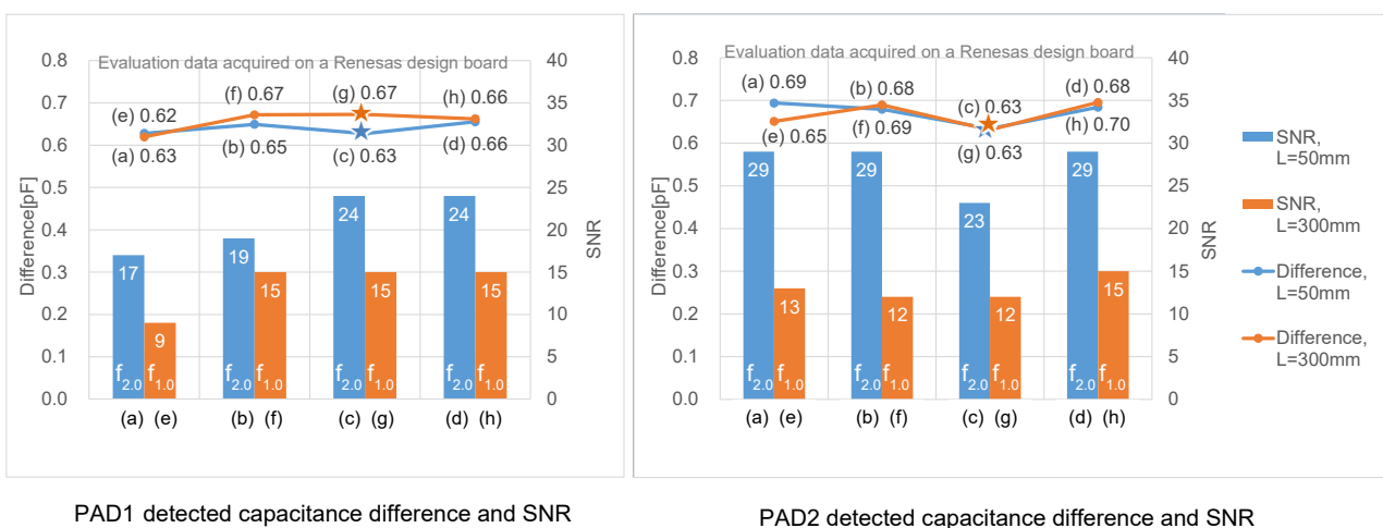
Figure 5-16 Wiring Pitch and Sensitivity Characteristics
