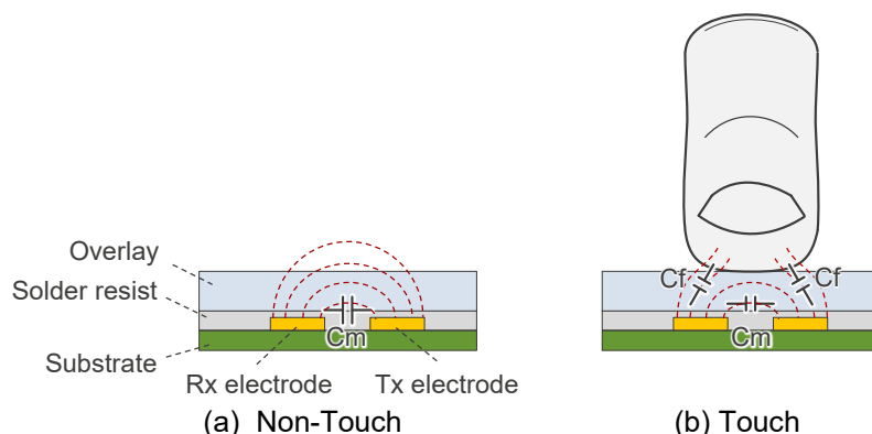
Figure3-2. Image of Mutual-capacitance Electrodes
