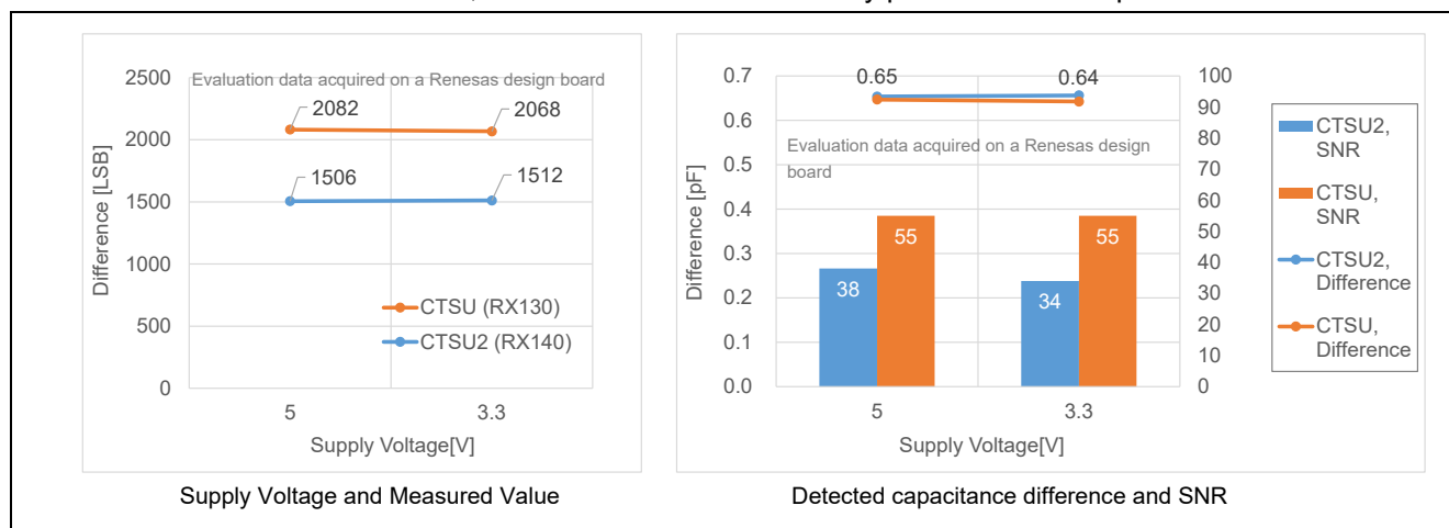
Figure 5-63 Normal Mode Supply Voltage and Sensitivity Characteristics
