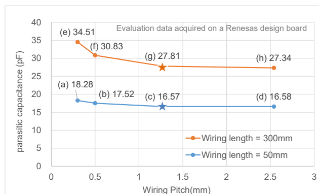
Figure 5-15 Wiring Pitch and Parasitic Capacitance (incl. CPU board)
