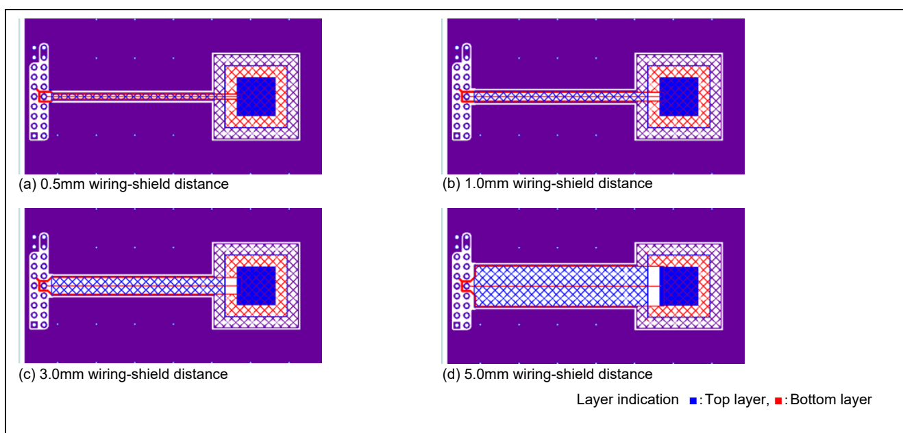
Figure 5-40 Evaluation Board Pattern (wiring-active shield distance)
