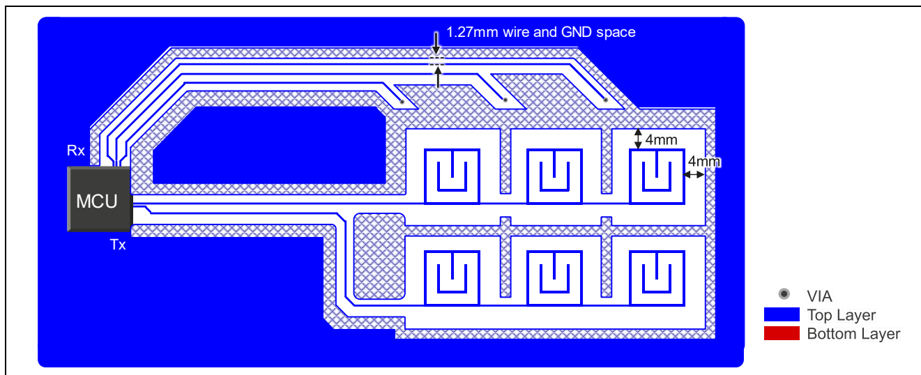
Figure3-14. Anti-noise Countermeasure Layout Pattern Example (top layer)
