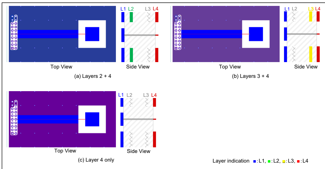
Figure 5-26 Evaluation Board Pattern (solid GND)
