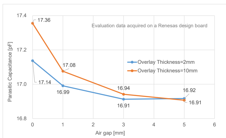
Figure 5-51 Overlay Air Gap and Parasitic Capacitance
