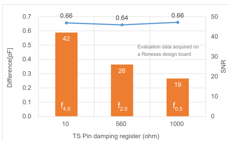
Figure 5-54 Damping Resistance Value and Sensitivity Characteristics
