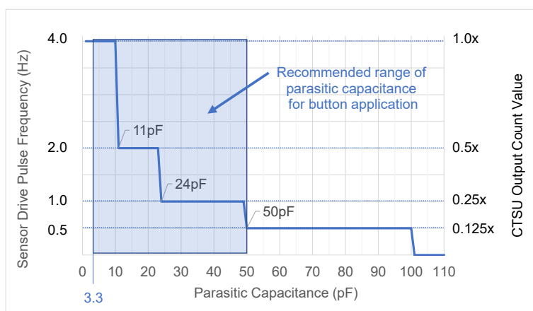
Figure 5-2 Setting Example for Parasitic Capacitance and Sensor Drive Pulse Frequency
