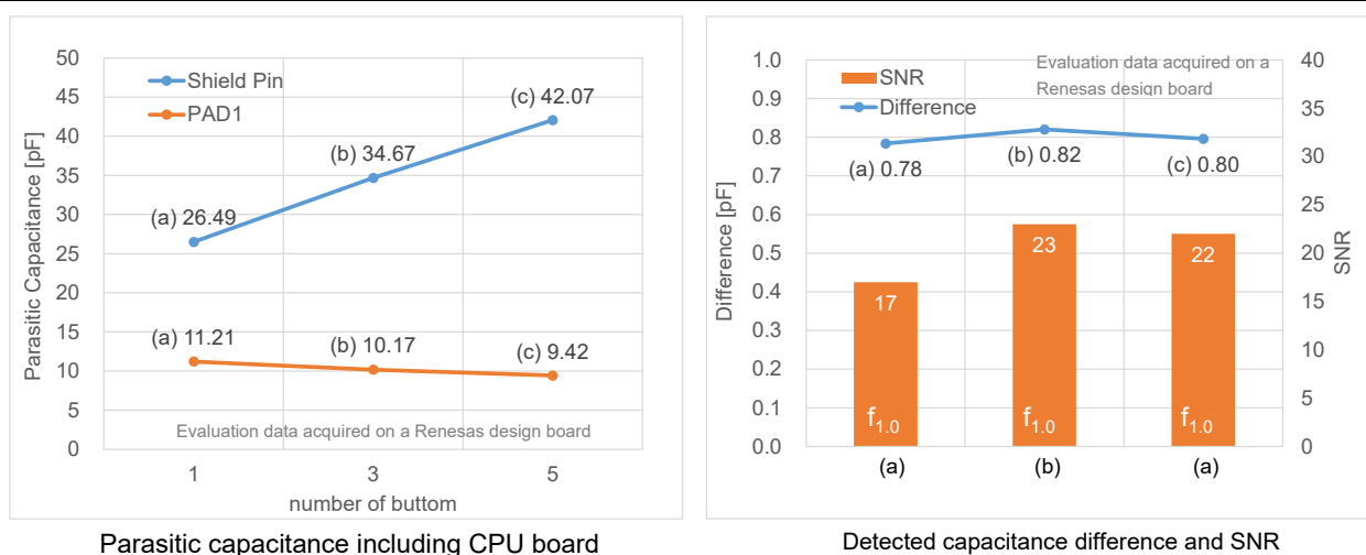
Figure 5-37 Active Shield Capacitance and Sensitivity Characteristics
