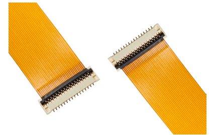
0.25mm-Pitch Premo-Flex Jumpers and Easy-On FPC Connectors
