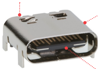
USB 4.0 Type-C Receptacle
