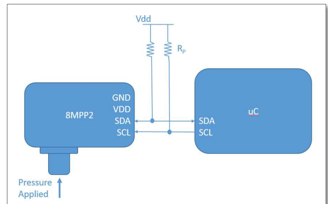
Figure 1-1: Digital I 2 C pressure sensor connected to a microcontroller
