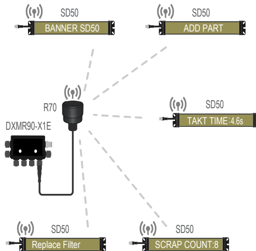
Example SD50 Wireless network layout (star topology)
