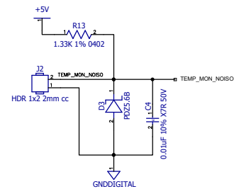
NON ISOLATED TEMP SENSOR
