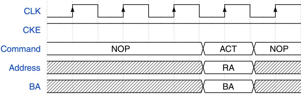
Figure 25-8. IP command - SDRAM ACTIVE
