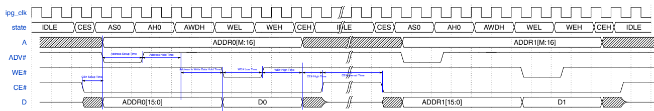
Figure 25-55. SRAM Write in ASYNC mode (ADMUX)
