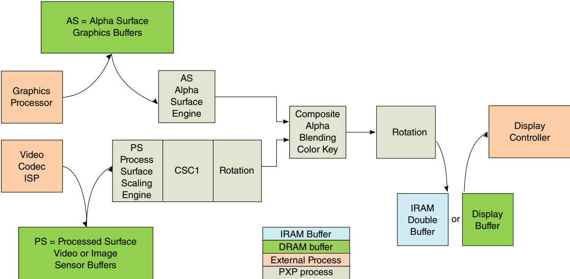
Figure 36-1. PXP Architecture
