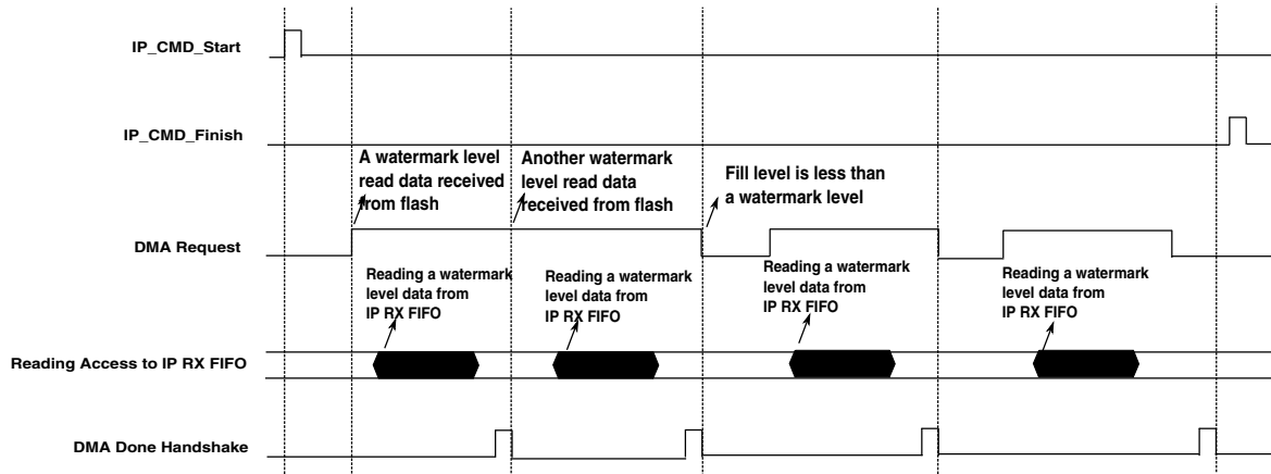
Figure 27-14. Reading from IP RX FIFO by DMA
