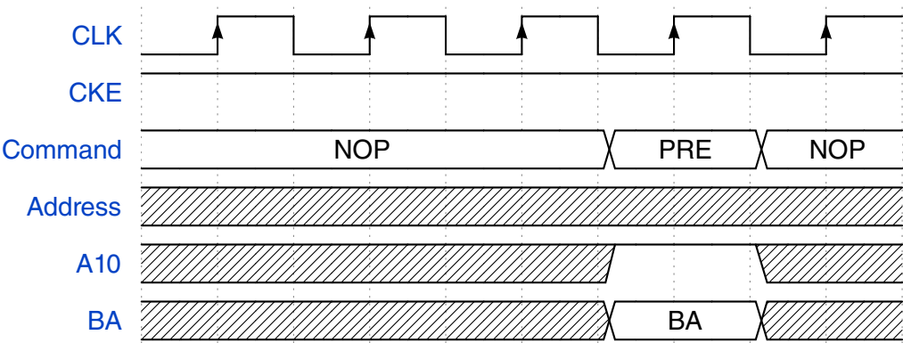
Figure 25-7. IP command - SDRAM PRECHARGE ALL
