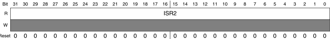
GPC_ISR2 field descriptions
