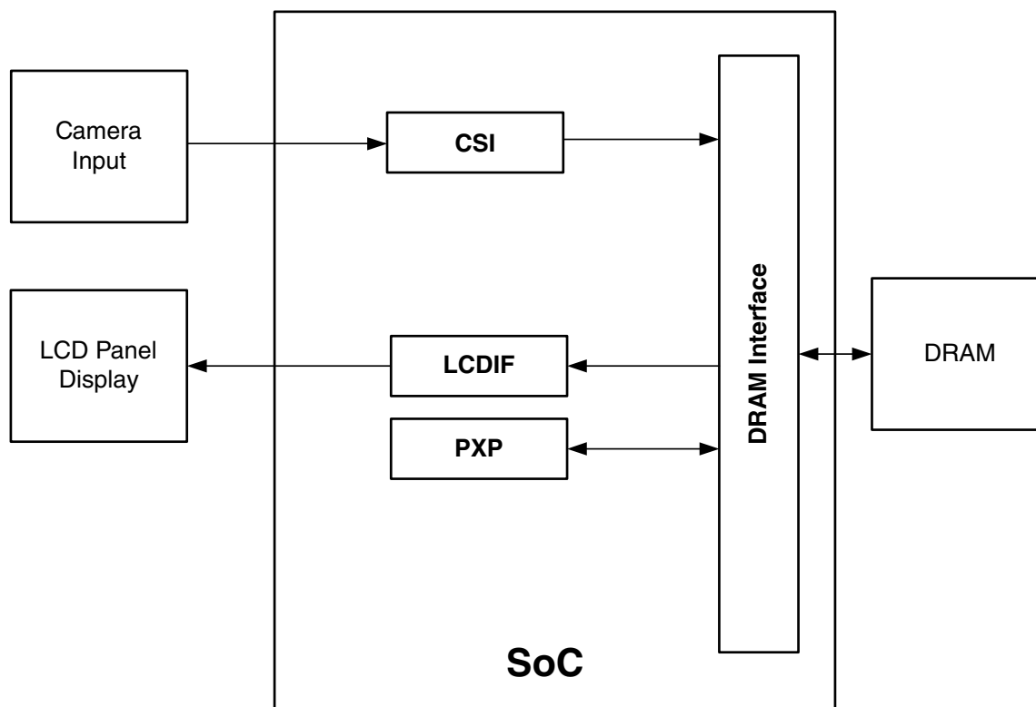
Figure 33-1. Block Diagram
