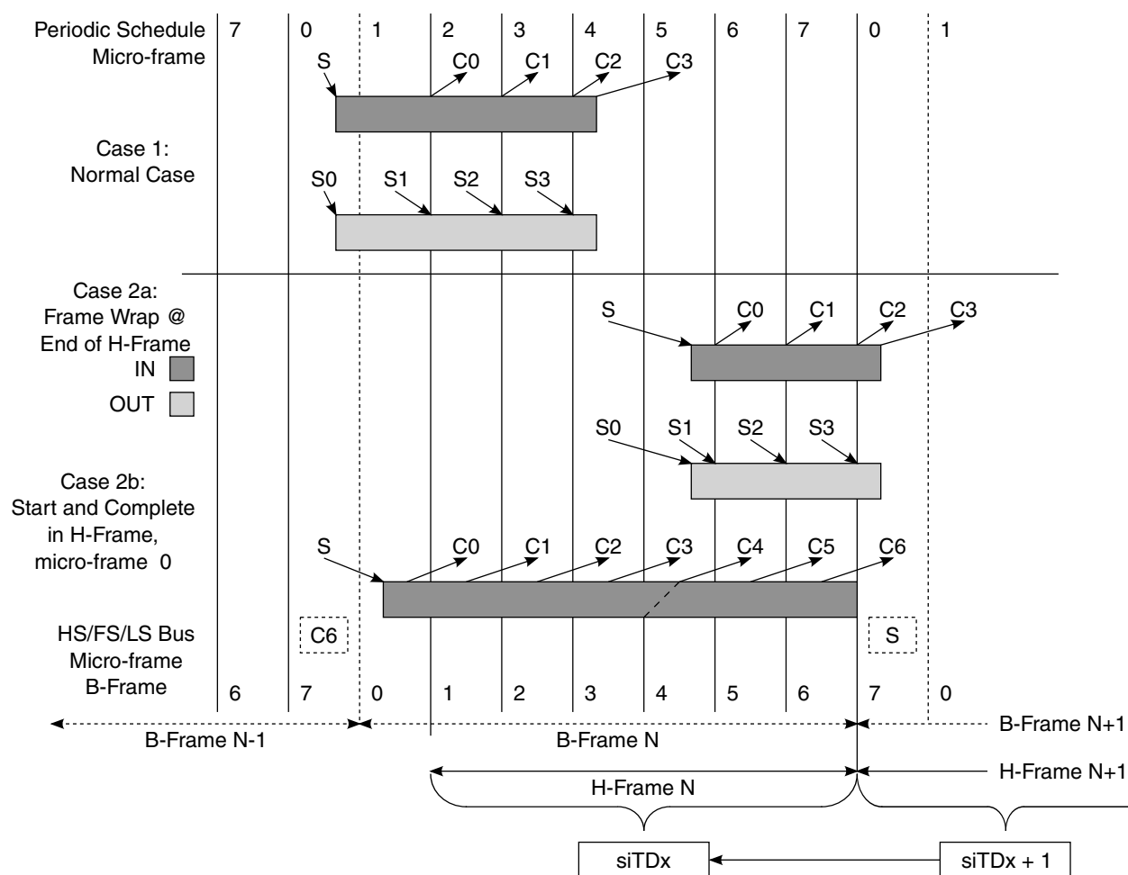
Figure 42-24. Split Transaction, Isochronous Scheduling Boundary Conditions
