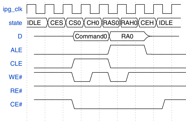
Figure 25-30. NAND Flash access Address type - One Byte Row Address
