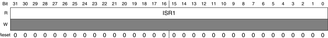
GPC_ISR1 field descriptions
