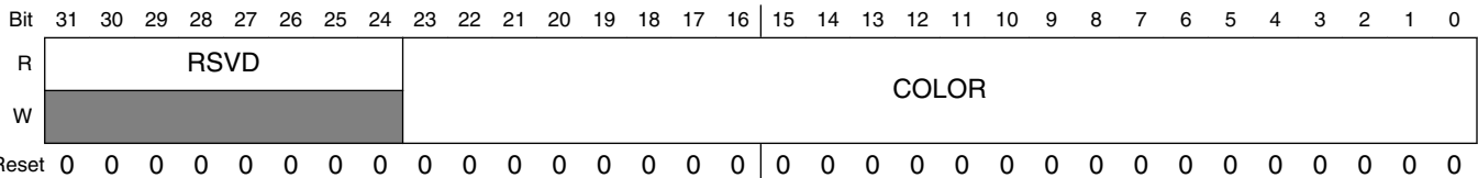
PXP_PS_BACKGROUND field descriptions
