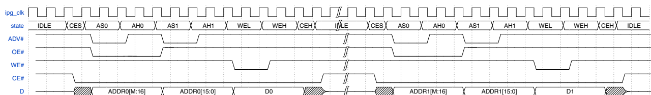
Figure 25-56. SRAM Write in ASYNC mode (AADM)
