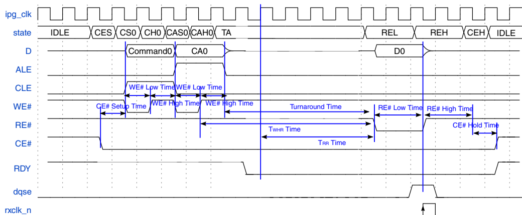
Figure 25-38. NAND Flash access command type - Command + Address + Read Phase
