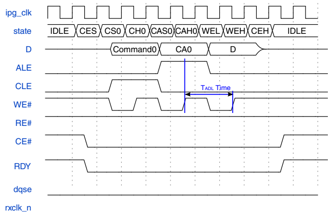
Figure 25-39. NAND Flash access command type - Command + Address + Write Phase
