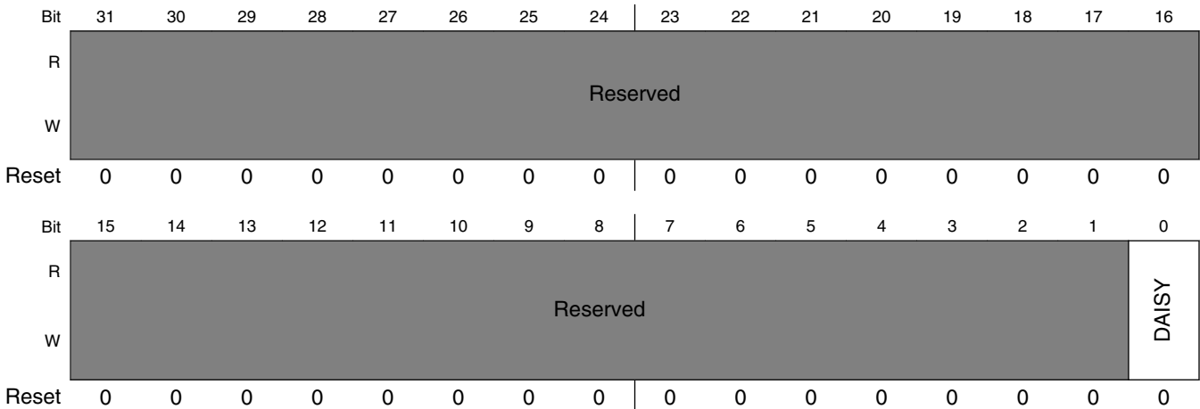
IOMUXC_NMI_SELECT_INPUT field descriptions
