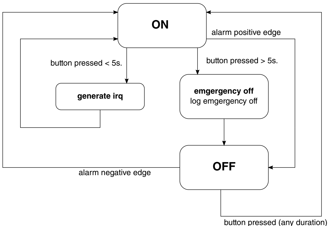
Figure 21-4. FSM
