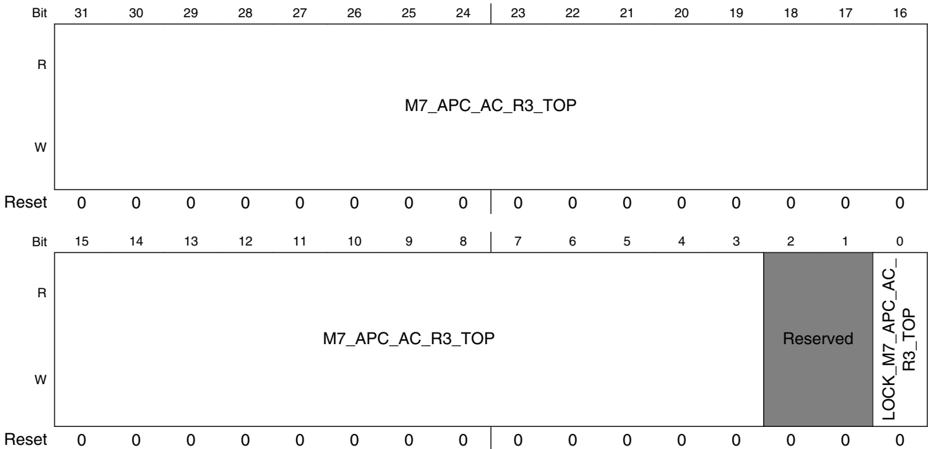
IOMUXC_GPR_GPR25 field descriptions
