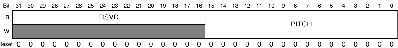
PXP_AS_PITCH field descriptions
