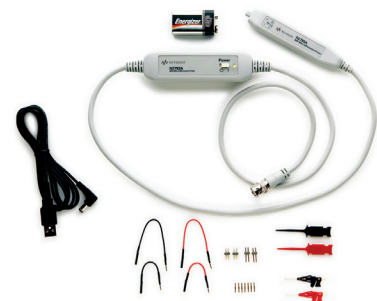
N2793A 800-MHz, 15-V differential probe
