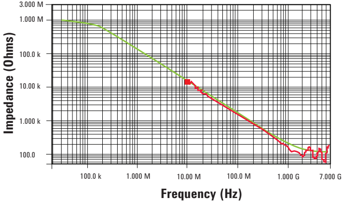
Input impedance over frequency (Red = measured, Green = model)
