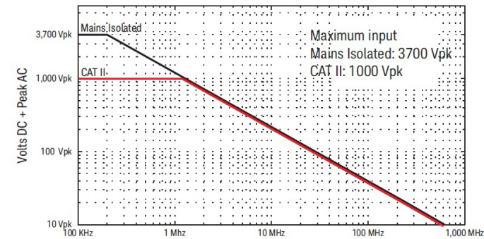
10076C derating curve
