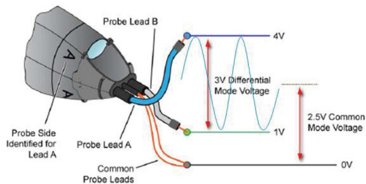
The N2750A Series InfiniiMode differential probes are a new generation of low-cost, 1.5, 3.5, and 6 GHz differential active probes compatible with Infiniium oscilloscope's AutoProbe interface
