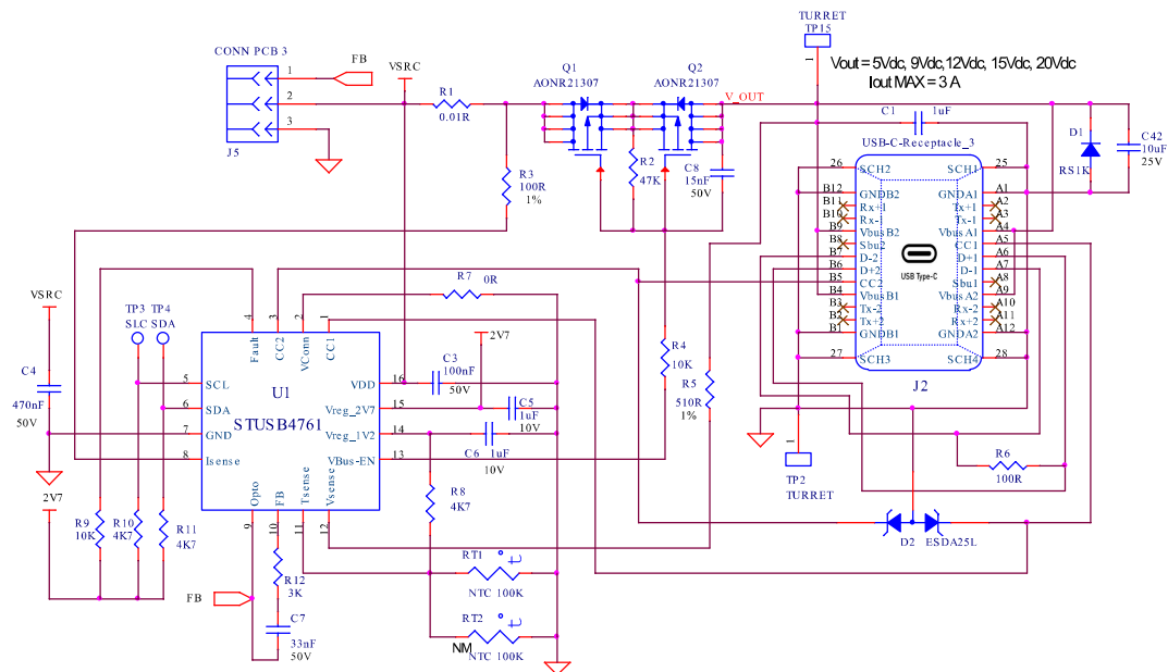
Daughterboard circuit schematic
