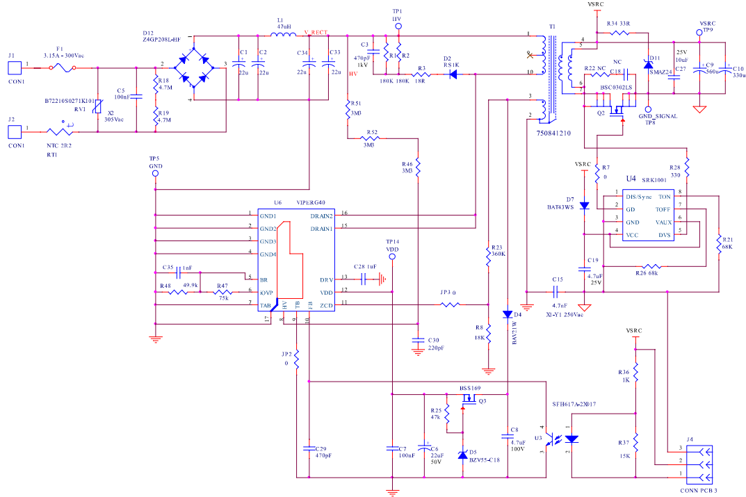
Daughterboard circuit schematic
