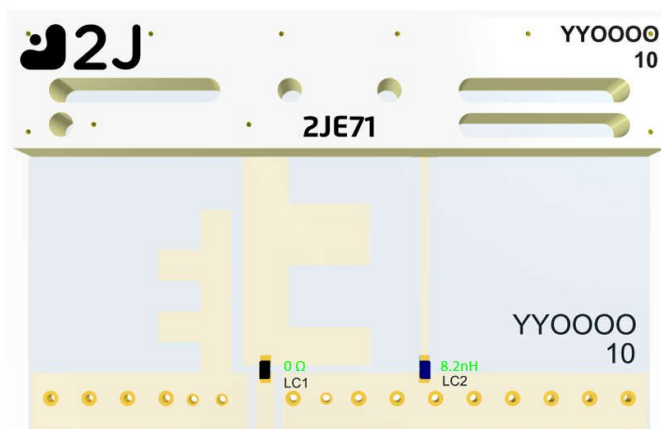
3D View of matching components and recommended values (LC1=0 Ohm, LC2=8.2nH)
