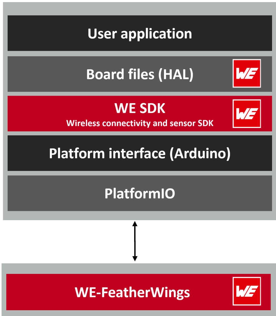
Figure 11: Software architecture
