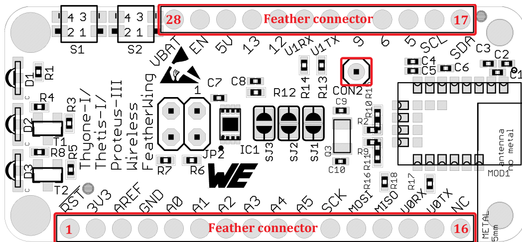
Figure 3: Connectors
