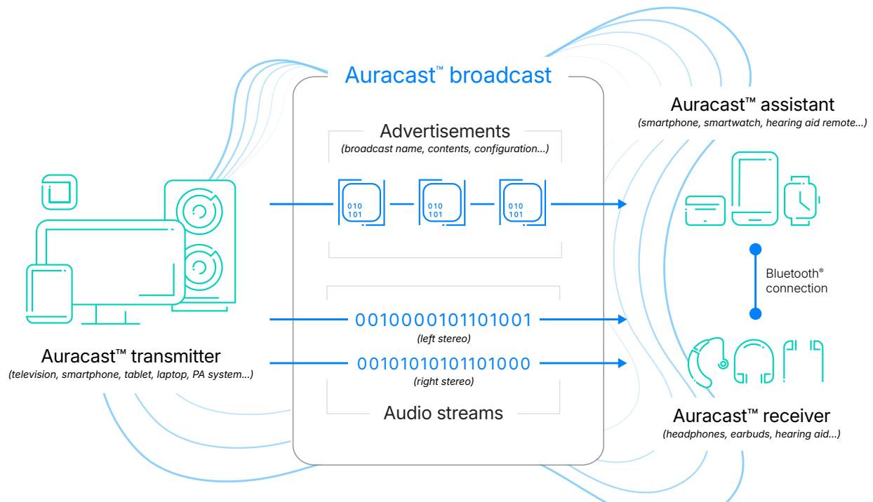
Figure 1.3 The basic topology of Auracast™ broadcast audio
