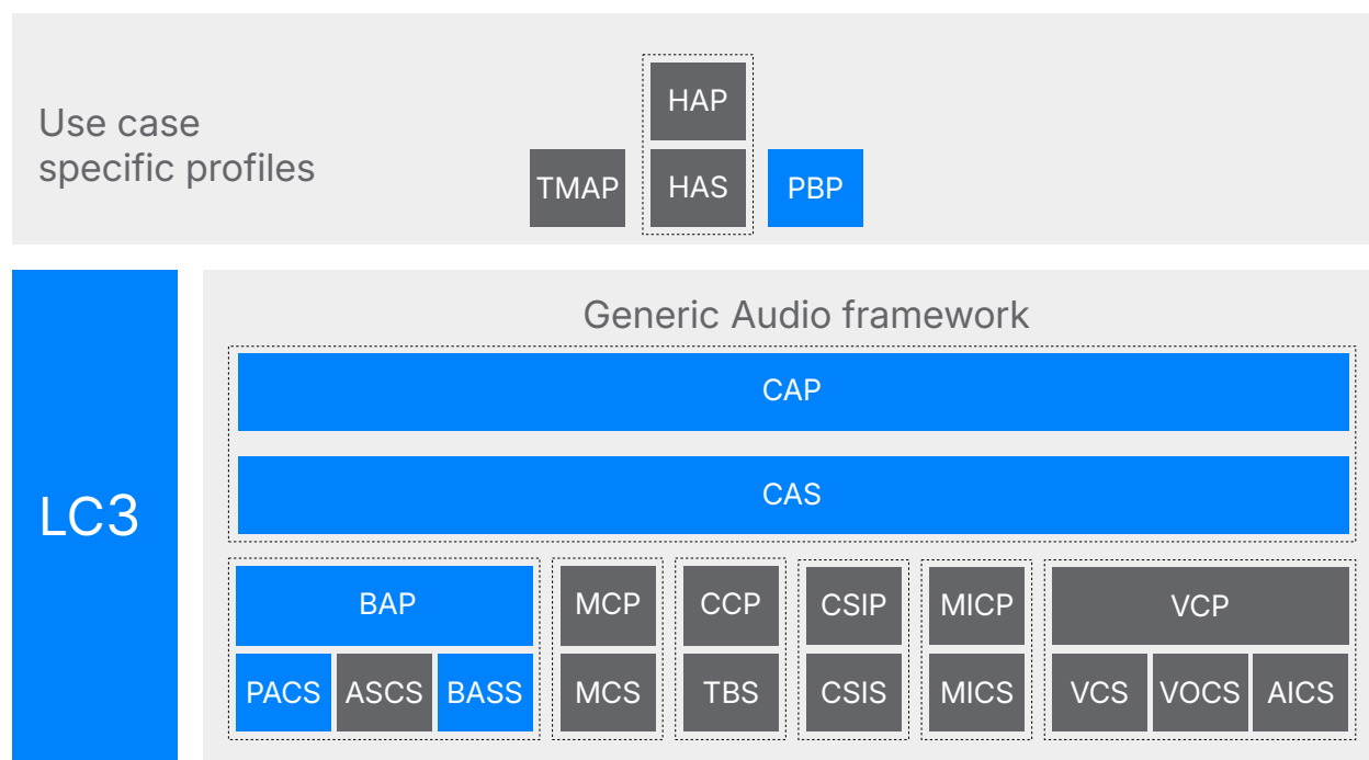
Figure 1.2: The Bluetooth LE Audio specifications required for Auracast™ devices
