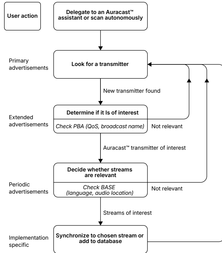
Figure 2.2: Basic scanning process
