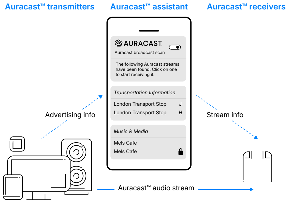
Figure 1.4: Data flow in Bluetooth® LE Audio broadcast
