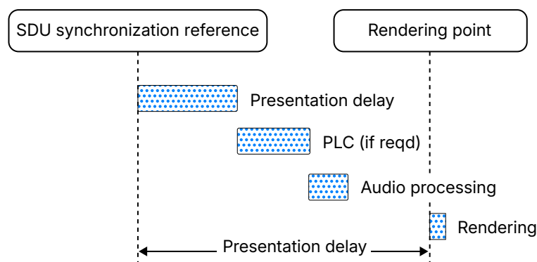
Figure 3.1: The use of Presentation Delay
