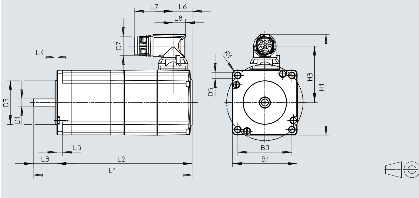
Dimensions – EMMT-ST
