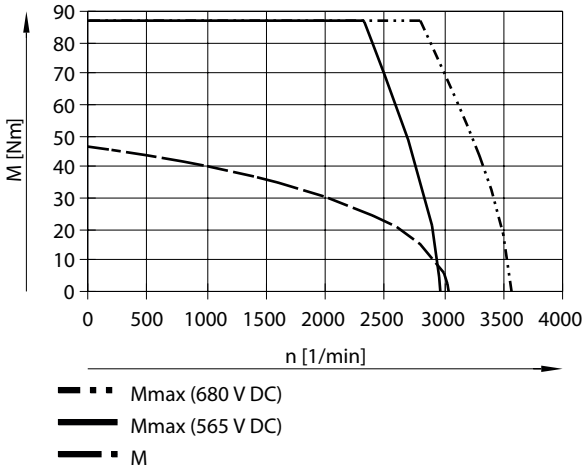
Torque M as a function of rotational speed n for EMMT-AS-150, long, high voltage, without/with brake
