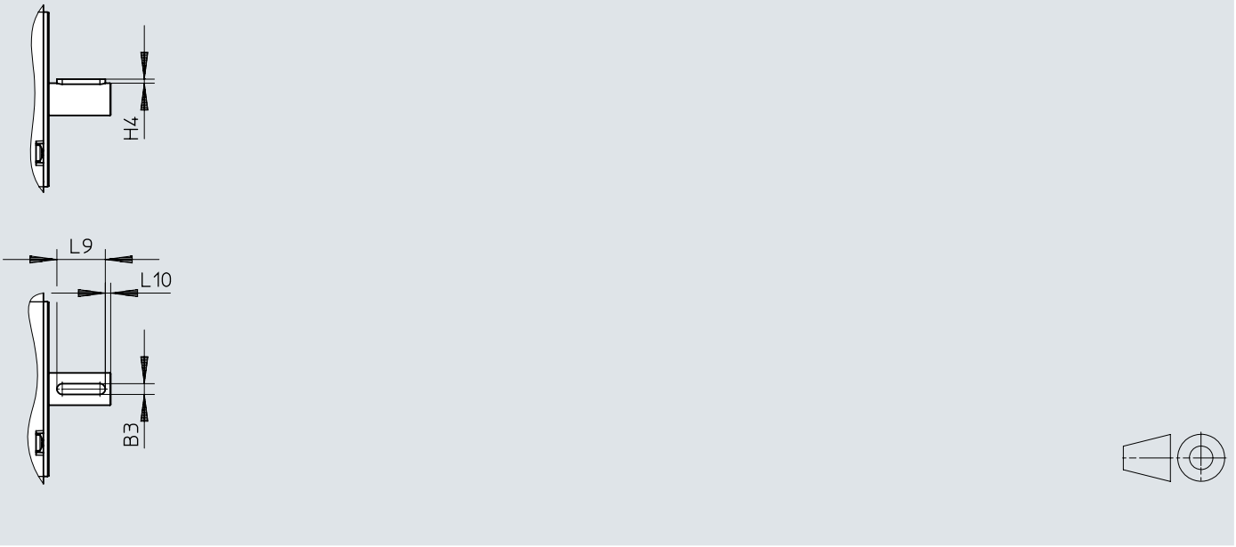
Dimensions – Featherkey for EMMT-AS-150, 190
