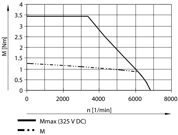
Torque M as a function of rotational speed n for EMMT-AS-60, medium, low voltage, without brake
