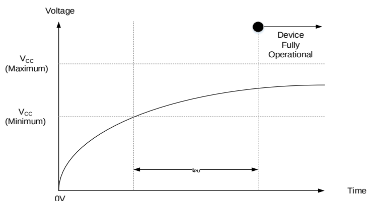
Figure 7: Power-Up Behavior
