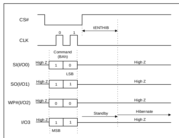
Figure 47: Enter Hibernate in QPI Command Sequence
