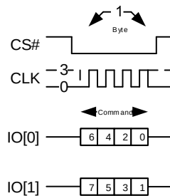
Figure 17: Description of (2-0-2) Instruction Type
