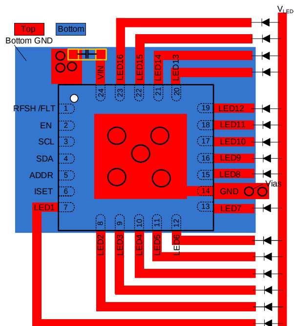
Figure 8: Recommended PCB Layout
