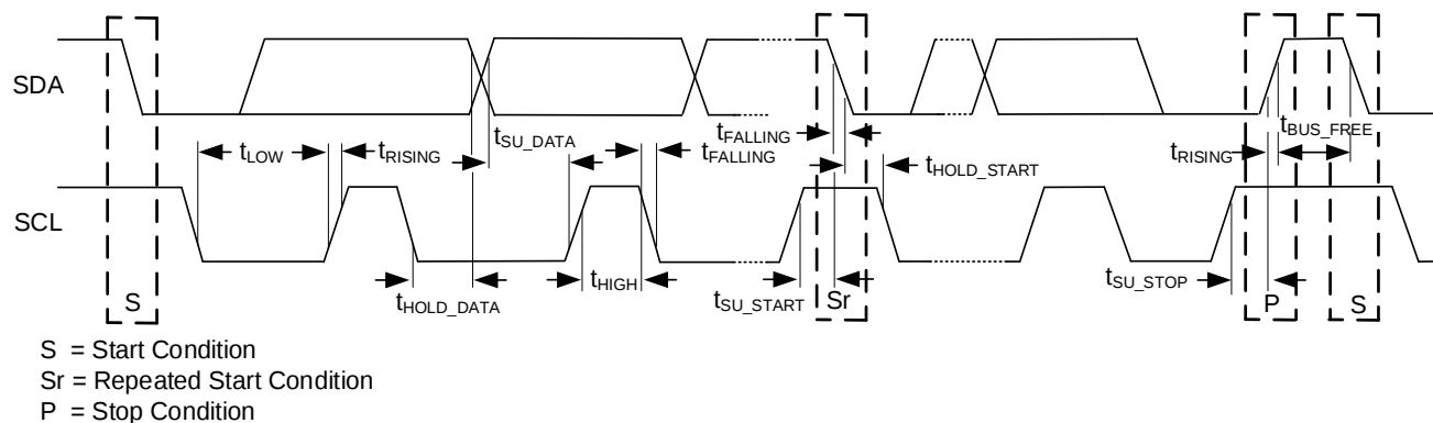
Figure 4: Digital Interface Timing Diagram
