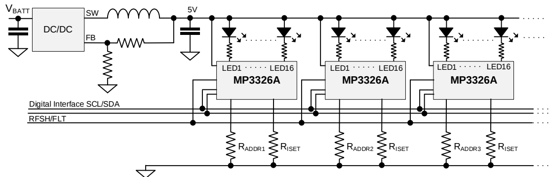
Figure 3: System Application Circuit with 1 LED and 1 Resistor in Series
