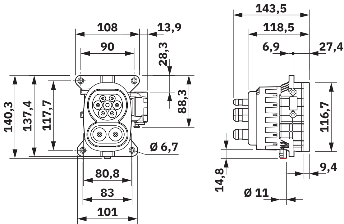
Dimensional drawing
