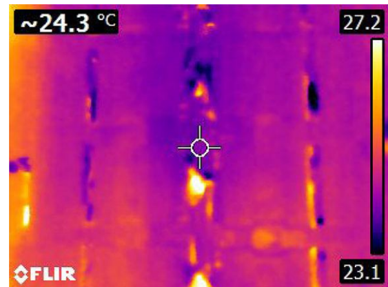
Fig. 22 - Stress Test With 20 A
