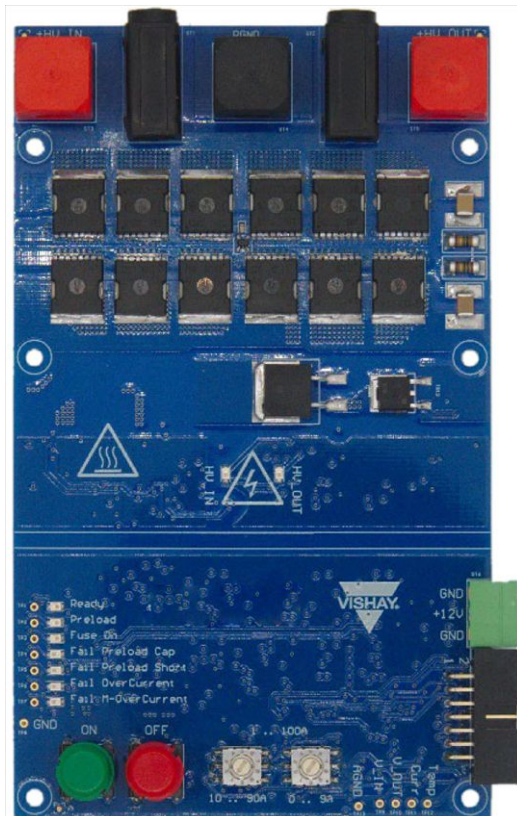
Fig. 1 - Vishay eFuse 400 V DC , 100 A (Top View)
