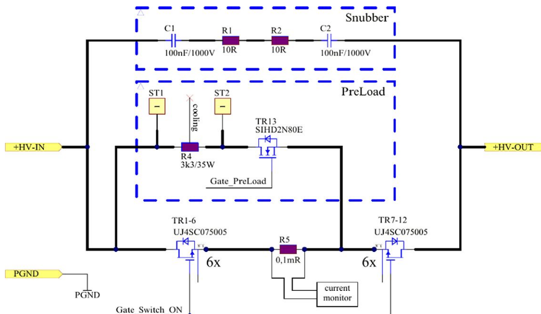
Fig. 3 - Overview of the High Voltage Side
