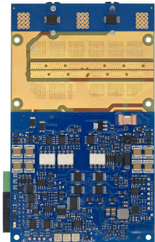
Fig. 2 - Vishay eFuse 400 V DC , 100 A (Bottom View)
