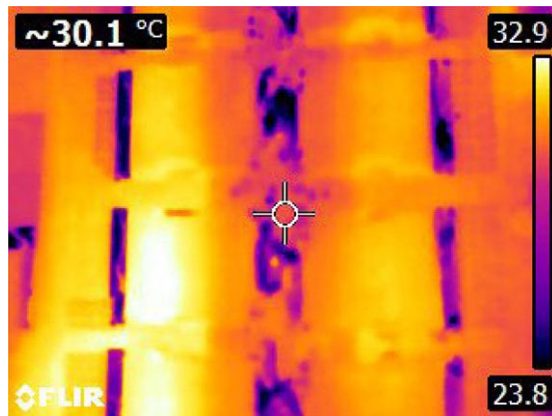
Fig. 23 - Stress Test With 50 A
