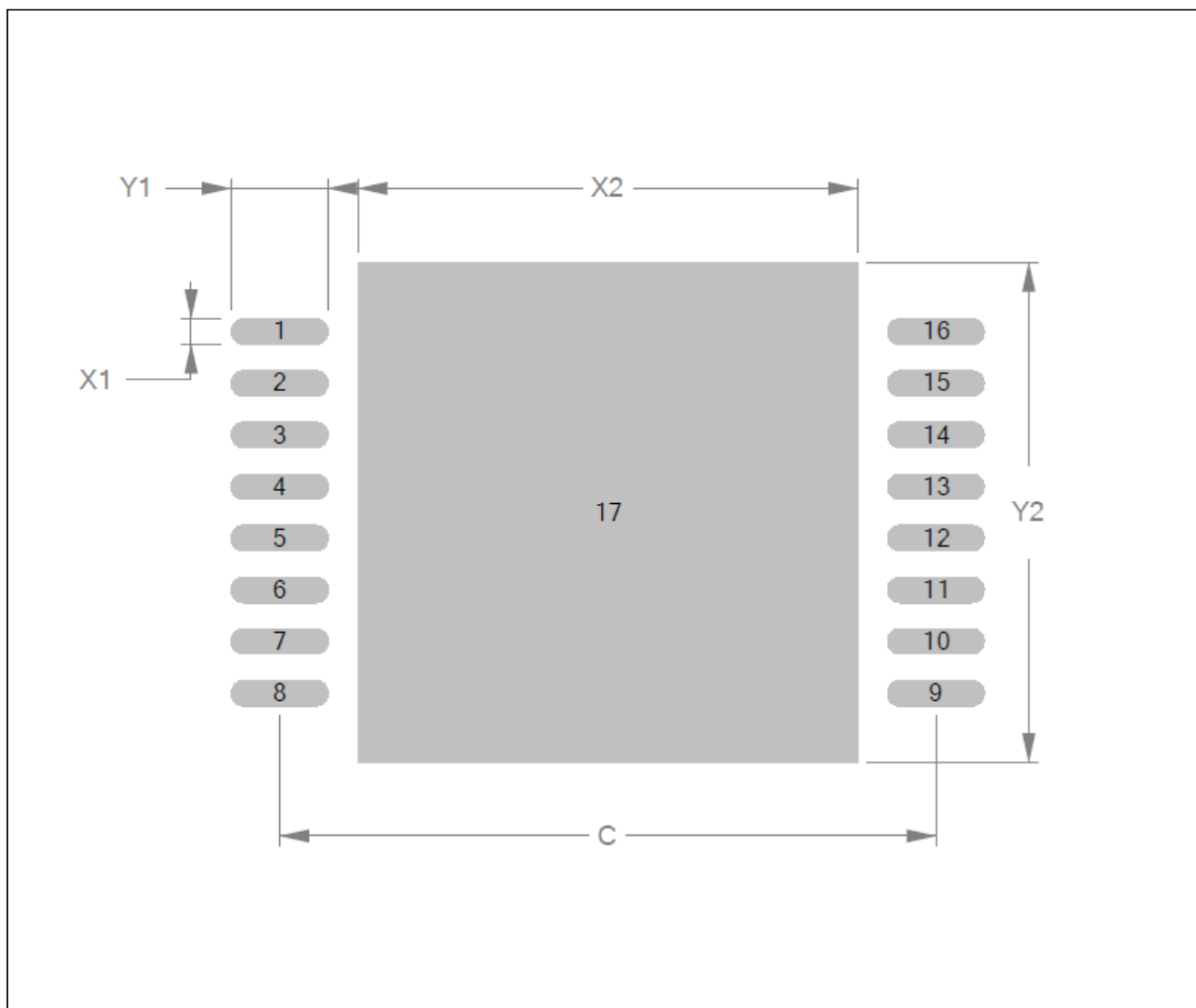
Figure 2-2. Recommended Land Pattern
