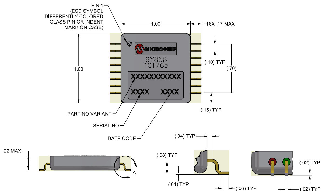
Figure 2-1. Outline Drawing
