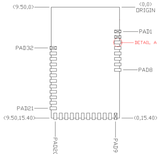
Figure 6. Solder Pad Reference Location
