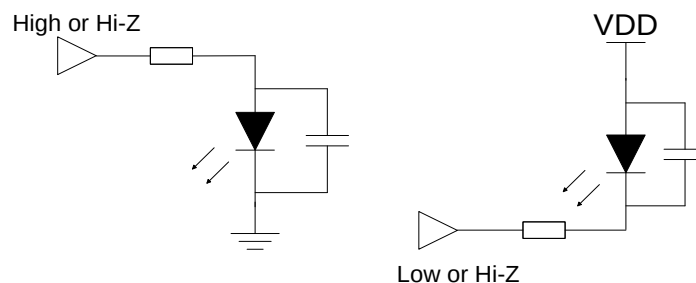
Figure 3-67. LED Circuits
