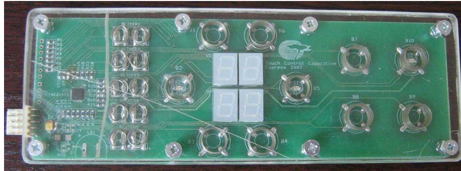
Figure 5-14. Cooktop Front Panel
