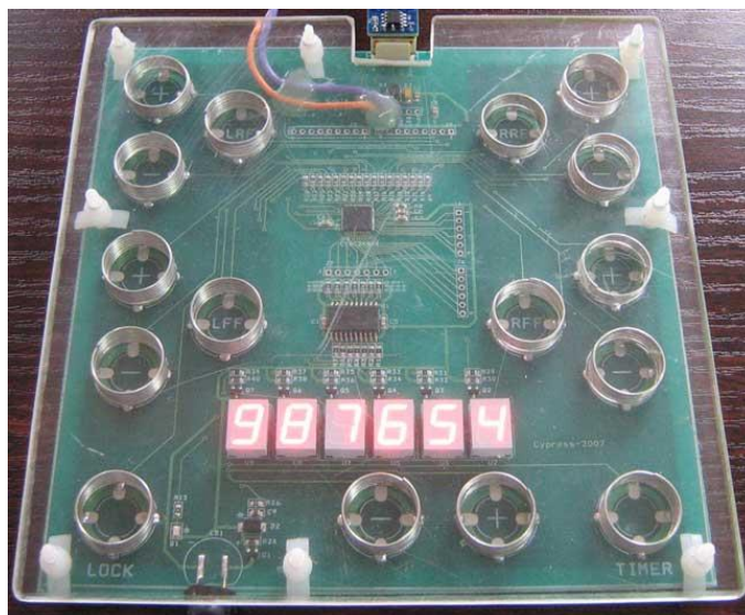
Figure 5-13. Demo Cooktop
