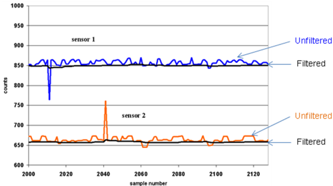
Figure 3-28. Median Filter Noise Spike
