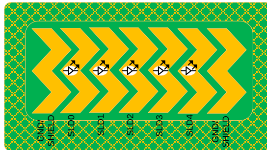
Figure 3-60. Slider Design with LED Backlighting
