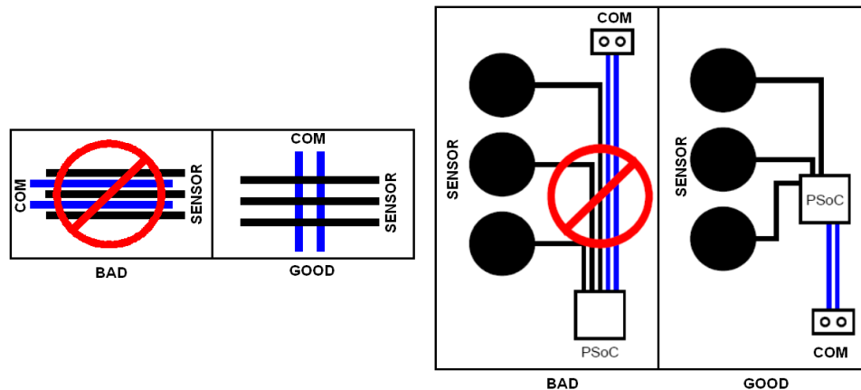
Figure 3-63. Routing of Sensing and Communication Lines
