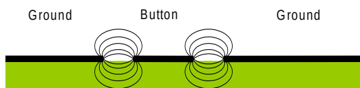
Figure C-2: Button-Ground Plane Fringing Fields
