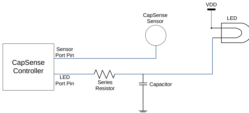
Figure 3-66. Filter Capacitor Solution for Crosstalk
