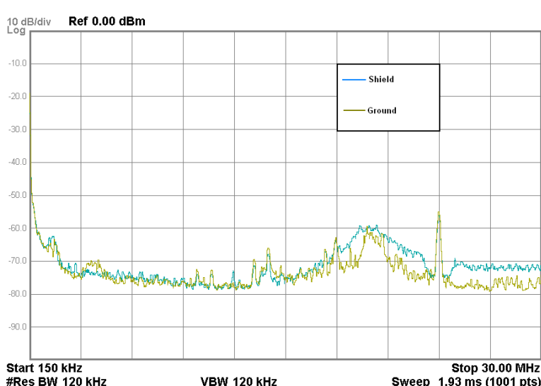
Figure 3-20. Effect of Inactive Sensor Termination
