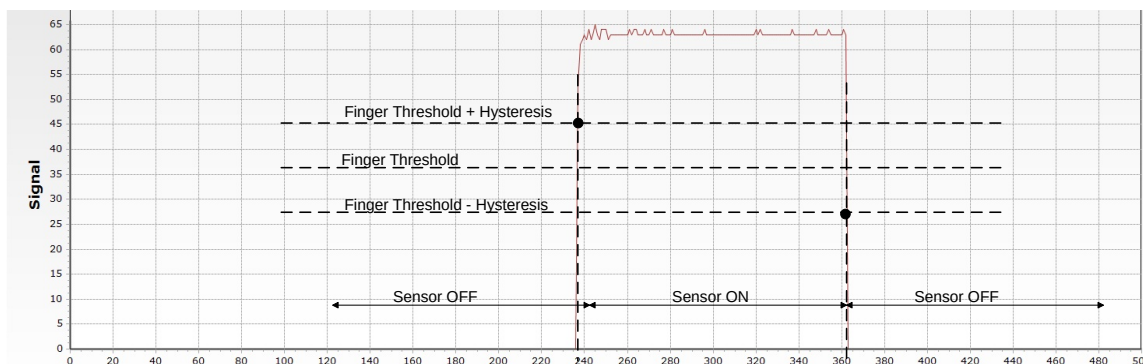
Figure 2-16. Hysteresis
