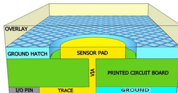
Figure 3-61. CapSense Design on 2-Layer PCB
