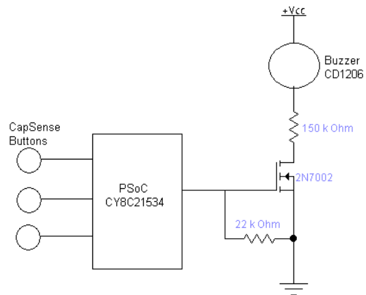
Figure 2-49. Implementing Audible Feedback for CapSense
