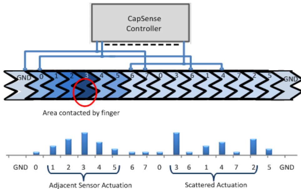
Figure 2-25. 16-Segment Diplexed Slider
