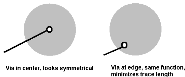
Figure 3-68. Via Placement on Sensor Pad
