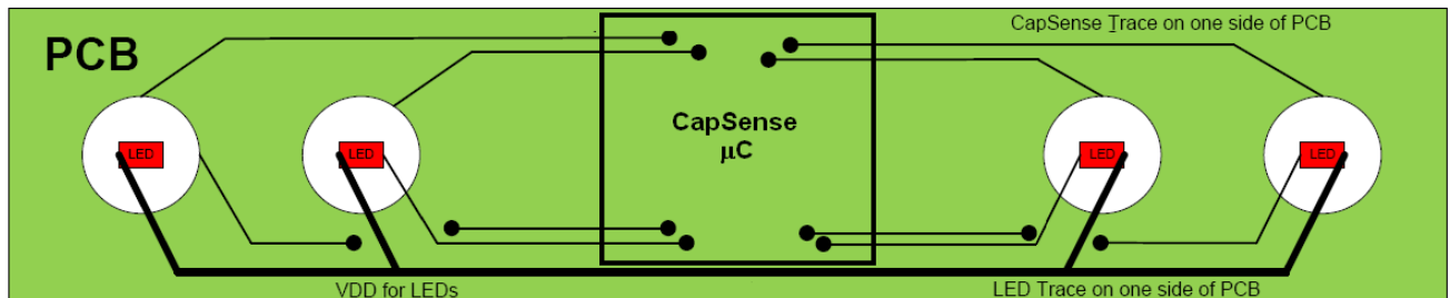
Figure 3-65. Recommended - LED and CapSense with Wide Separation
