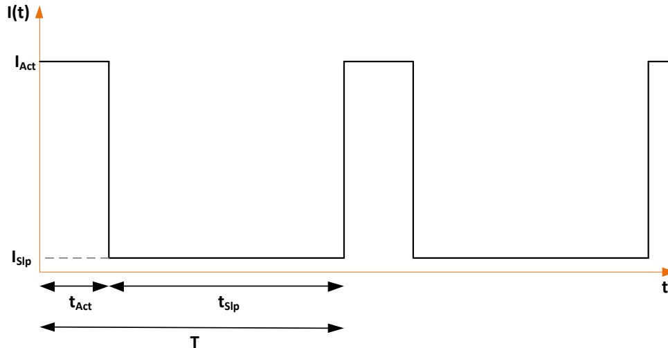
Figure 3-33. Instantaneous Current
