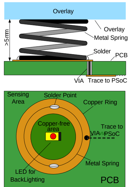
Figure 5-10. Spring-Mounting Example
