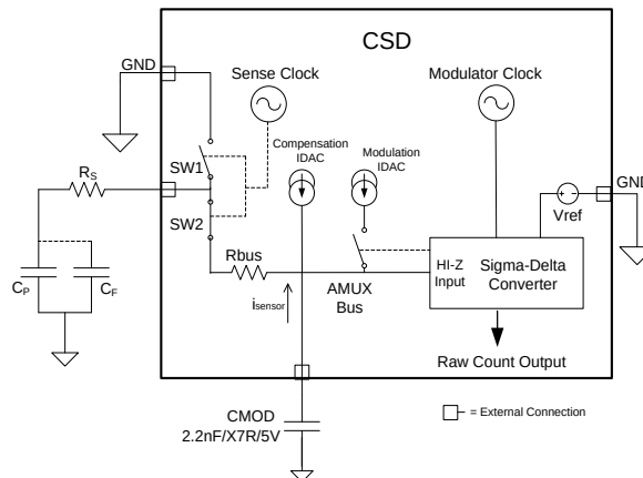
Figure 2-12. CSD Block Diagram
