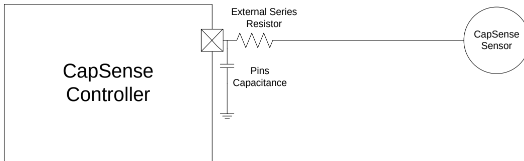
Figure 3-5. RC Filter
