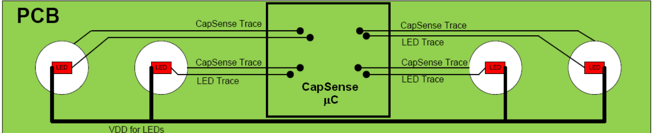
Figure 3-64. Not Recommended - LED and CapSense in Close Proximity
