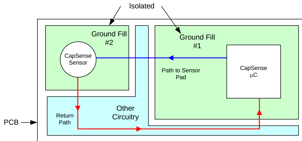
Figure 3-9. Improper Current Loop Layout
