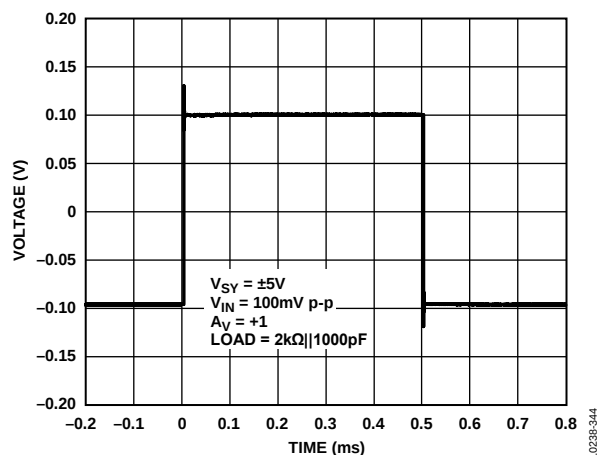
Figure 47. Small Signal Transient Response, V_{SV} = \pm 5\text{ V}
