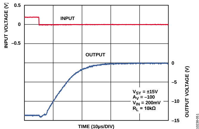
Figure 52. Negative Overload Recovery, V_{SV} = \pm 15\text{ V}
