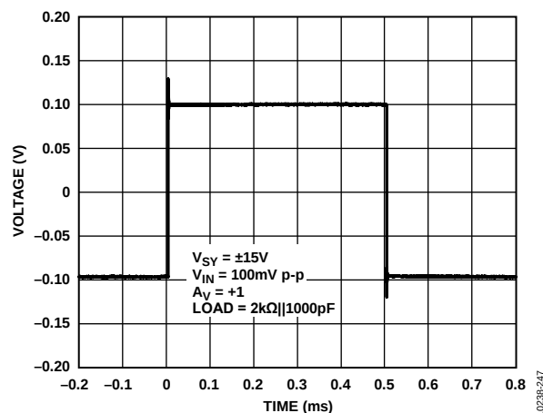
Figure 50. Small Signal Transient Response, V_{SV} = \pm 15\text{ V}
