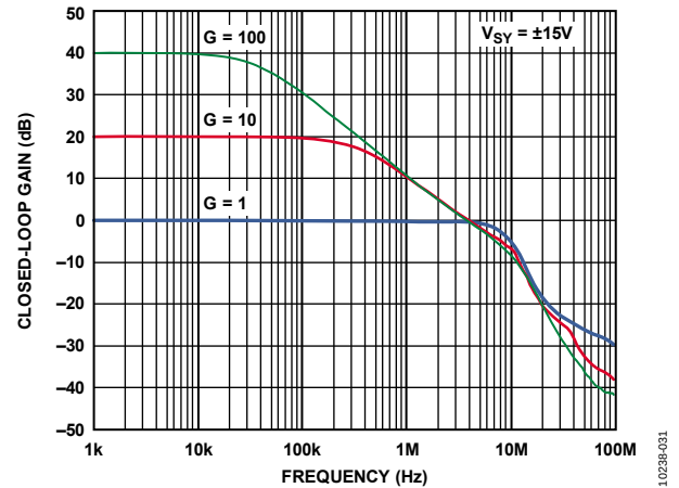
Figure 44. Closed-Loop Gain vs. Frequency, V_{SY} = \pm 15\text{ V}
