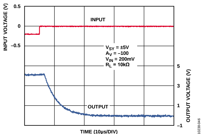
Figure 48. Positive Overload Recovery, V_{SV} = \pm 5\text{ V}
