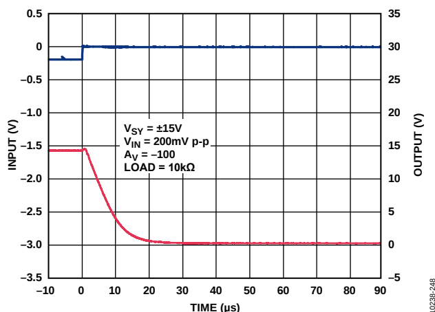
Figure 51. Positive Overload Recovery, V_{SV} = \pm 15\text{ V}
