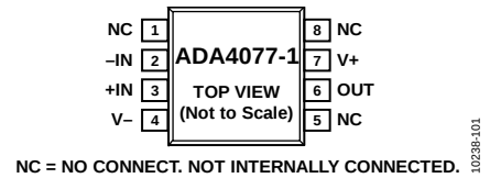
Figure 1. ADA4077-1, 8-Lead SOIC (and 8-Lead MSOP)
