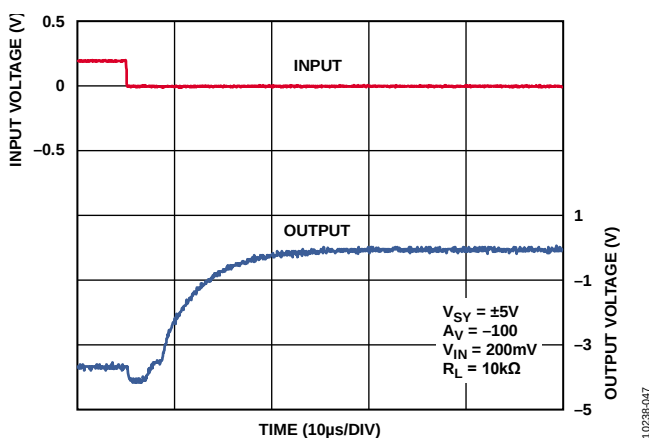
Figure 49. Negative Overload Recovery, V_{SV} = \pm 5\text{ V}
