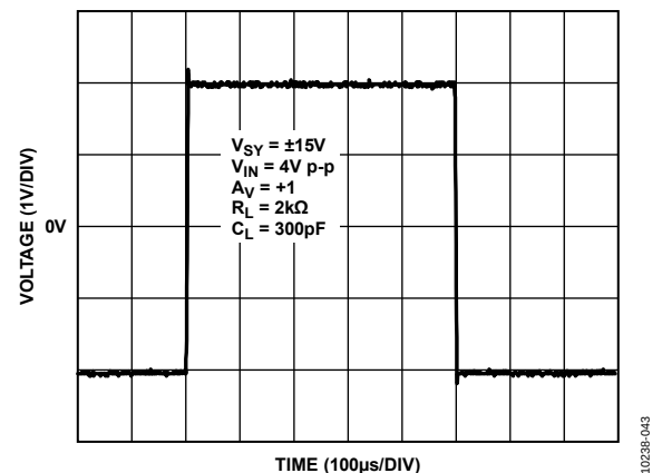
Figure 46. Large Signal Transient Response, V_{SY} = \pm 15\text{ V}
