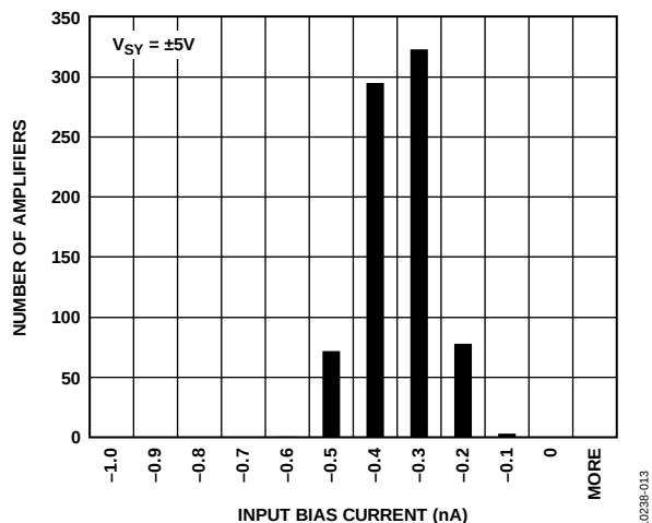
Figure 24. Input Bias Current, V_{SY} = \pm 5V
