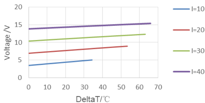
Performance Curves at T_h=27^\circ\text{C}
