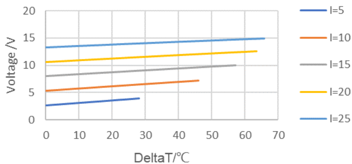
Performance Curves at T_h=27^\circ\text{C}
