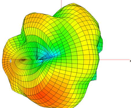
MIMO 1 – 30cmx30cm Ground Plane
