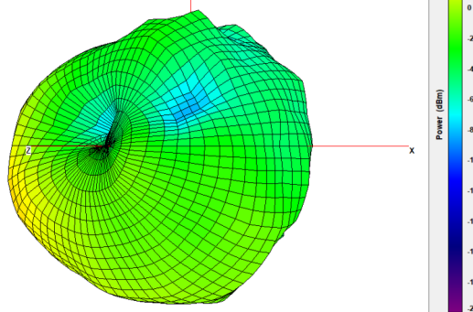
MIMO 2 – Free Space
