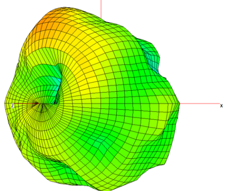
MIMO 1 – Free Space
