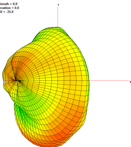
MIMO 1 – Free Space
