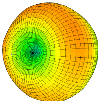
MIMO 1 – 30cmx30cm Ground Plane
