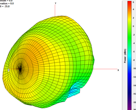
MIMO 1 – Free Space
