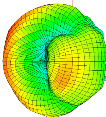
MIMO 1 – 30cmx30cm Ground Plane
