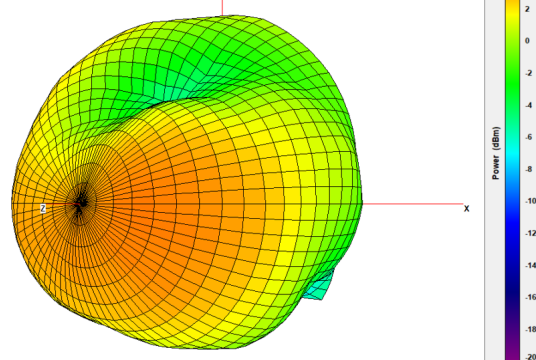
MIMO 1 – Free Space
