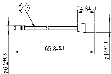
Whip Antenna-2(FW.79.M6.F): 700-900MHz Flexible Whip Antenna with M6 Female Connector
