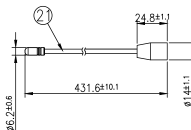
Whip Antenna-1(FW.19.M6.F): 150-174/430-520/700-900MHz Flexible Whip Antenna with M6 female connector
