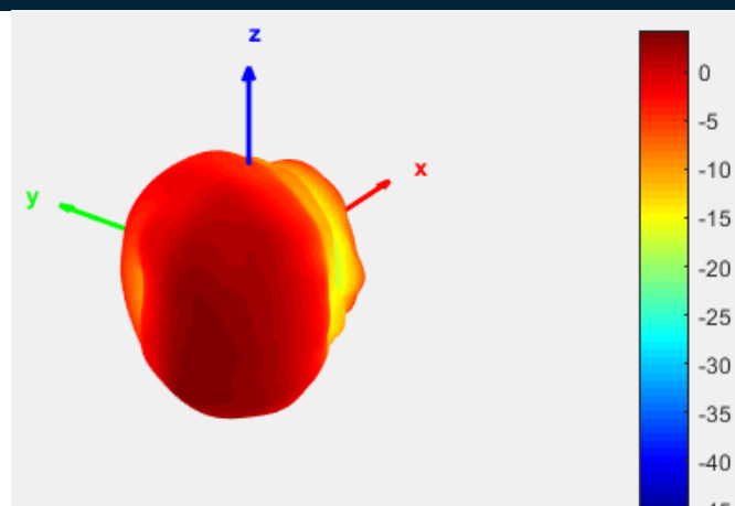
Radiation Pattern at 7.5GHz
