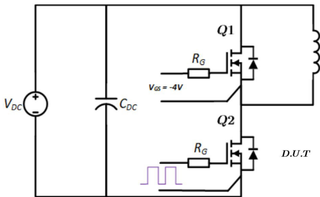
Figure 29. Clamped Inductive MOSFET Switching Waveform Test Circuit
