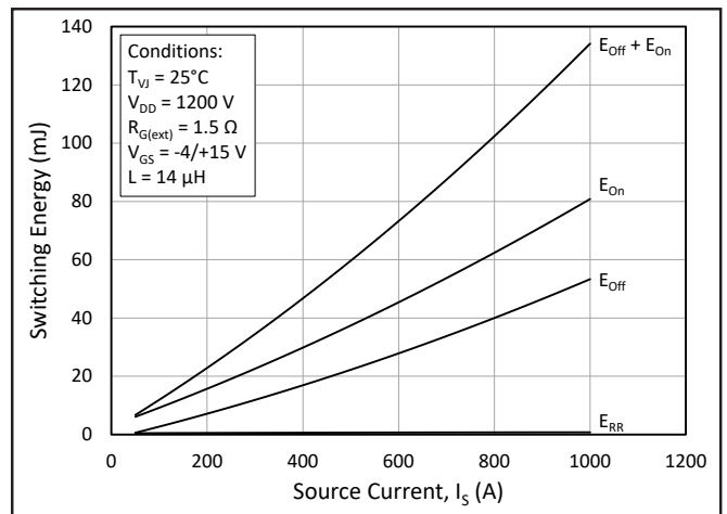
Figure 12. Switching Energy vs. Drain Current ( V_{DS} = 1200 V)
