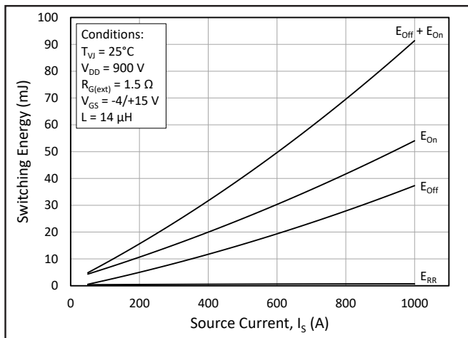
Figure 11. Switching Energy vs. Drain Current ( V_{DS} = 900 V)
