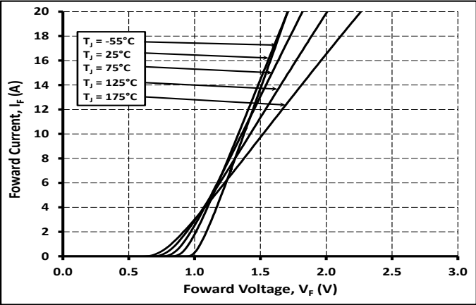
Figure 1 Forward Characteristics
