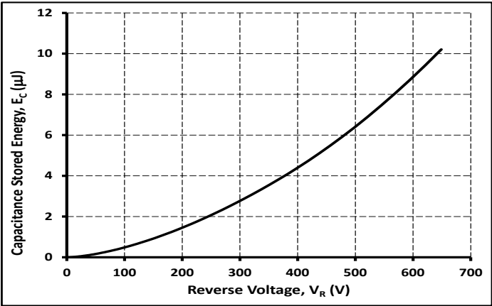
Figure 7 Capacitance Stored Energy
