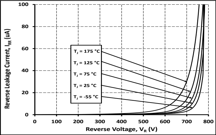
Figure 2 Reverse Characteristics
