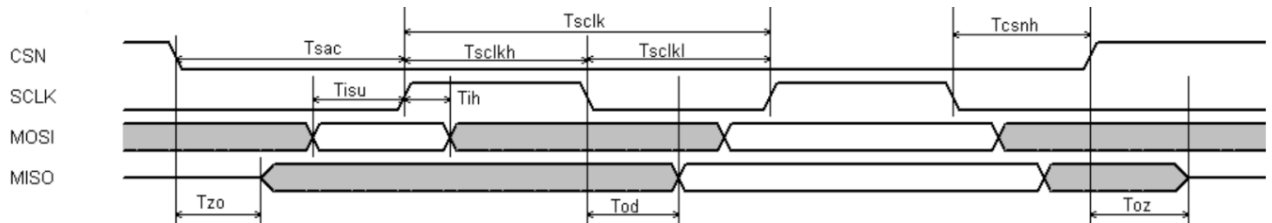
Figure 7. SPI timing diagram
