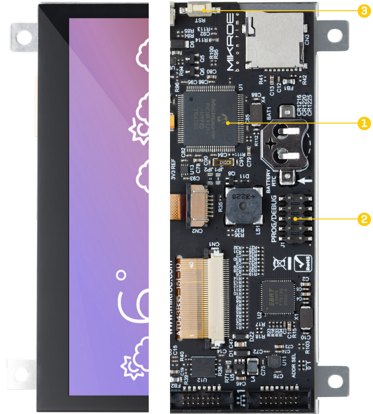
Figure 3: Front and back partial view
