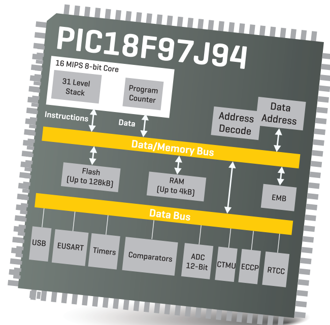
Figure 1: PIC18F97J94 MCU block schematic
