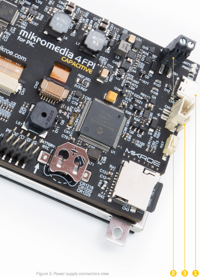
Figure 5: Power supply connectors view
