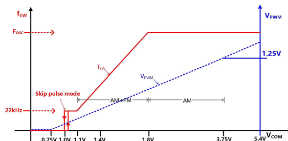
Fig. 14 Variation Curves of Switching Frequency and Peak Current with V_{COM}
