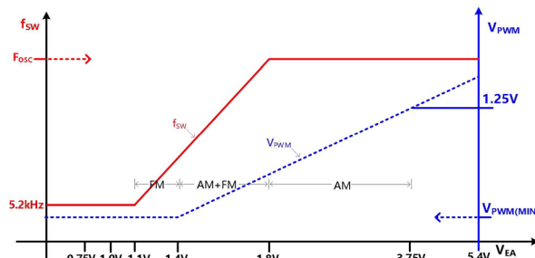
Fig. 13 Variation Curves of Switching Frequency and Peak Current with V_{EA}
