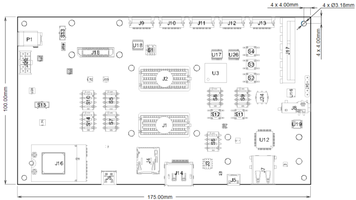
Figure 2: MitySOM-QC6490/5430 Development Kit Outline and Mounting Hole Locations (Top View, millimeters)
