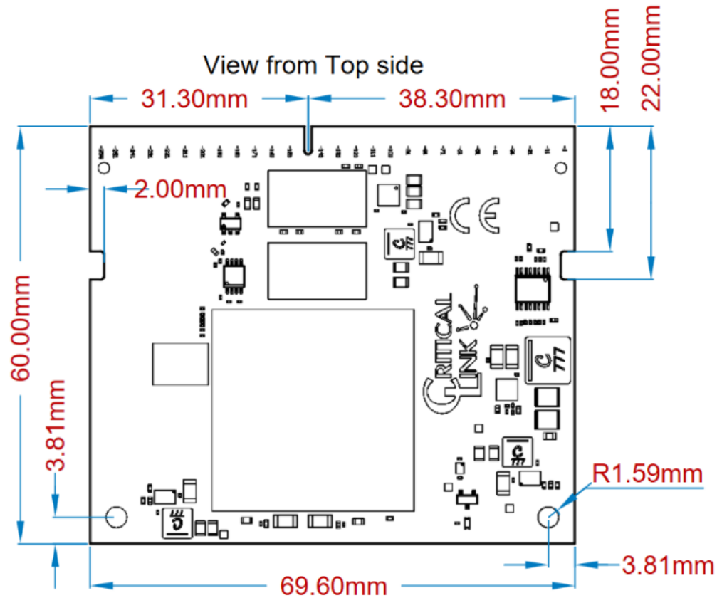
Figure 4 MitySOM-C10G Mechanical Outline, Top Side View
