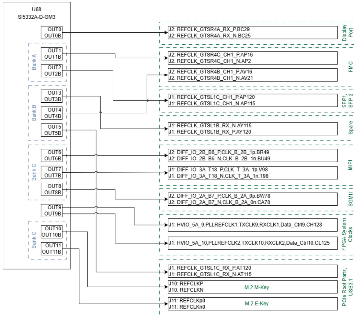
Figure 2 Clocking Topology
