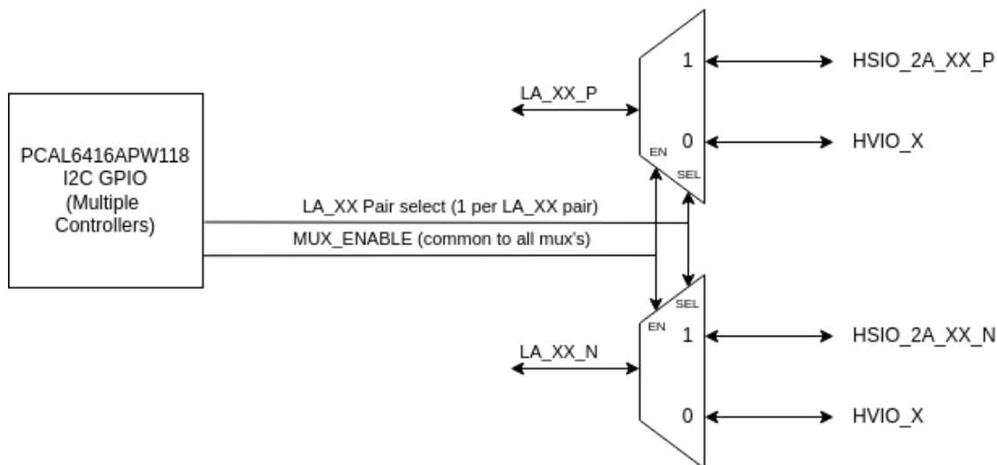
Figure 3 FMC LA_XX signal pair routing to HSIO or HVIO bank pins.
