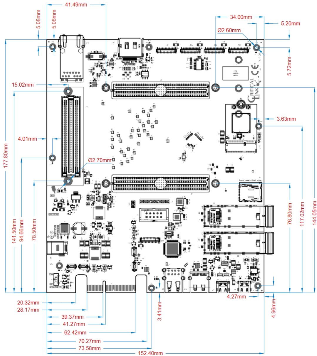
Figure 4: MitySOM-A5E Development Kit Outline and Mounting Hole Locations (Top View)
