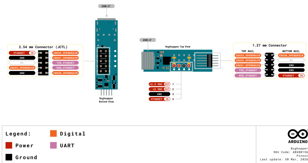
Bughopper pinout.
