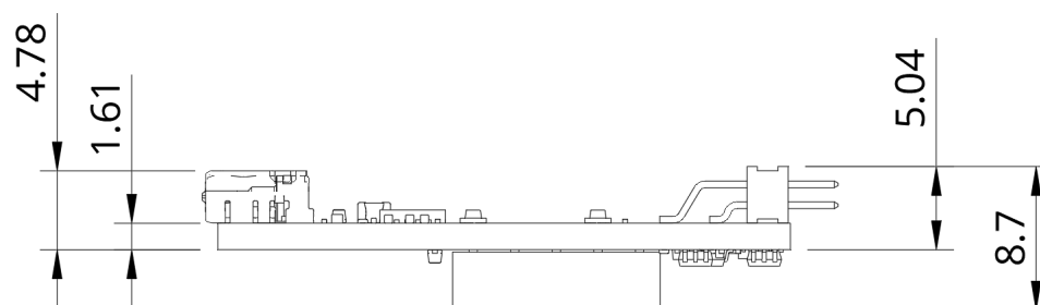
Bughopper board outline dimensions (side view); all dimensions are in mm.
