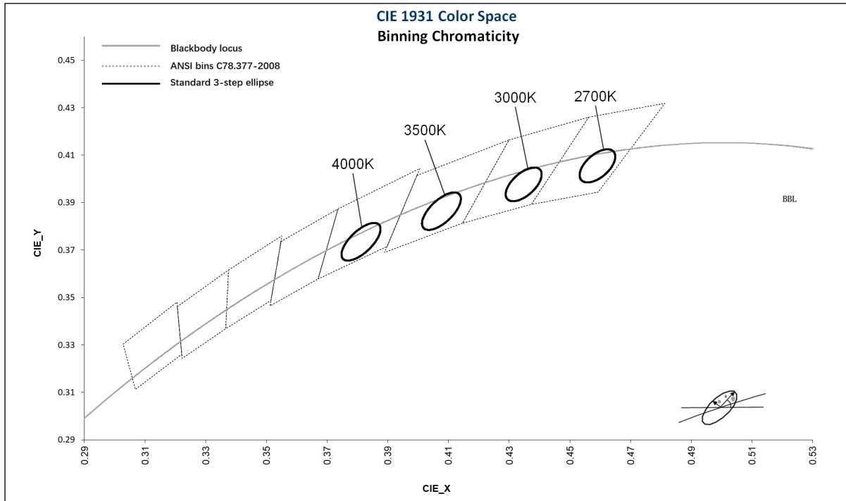
Chromaticity Binning Diagram 1 - TC61
