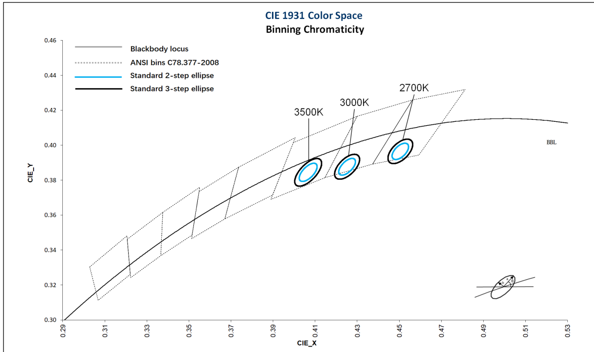
Chromaticity Binning Diagram 1 - TE62 Sensus (BBBL)
