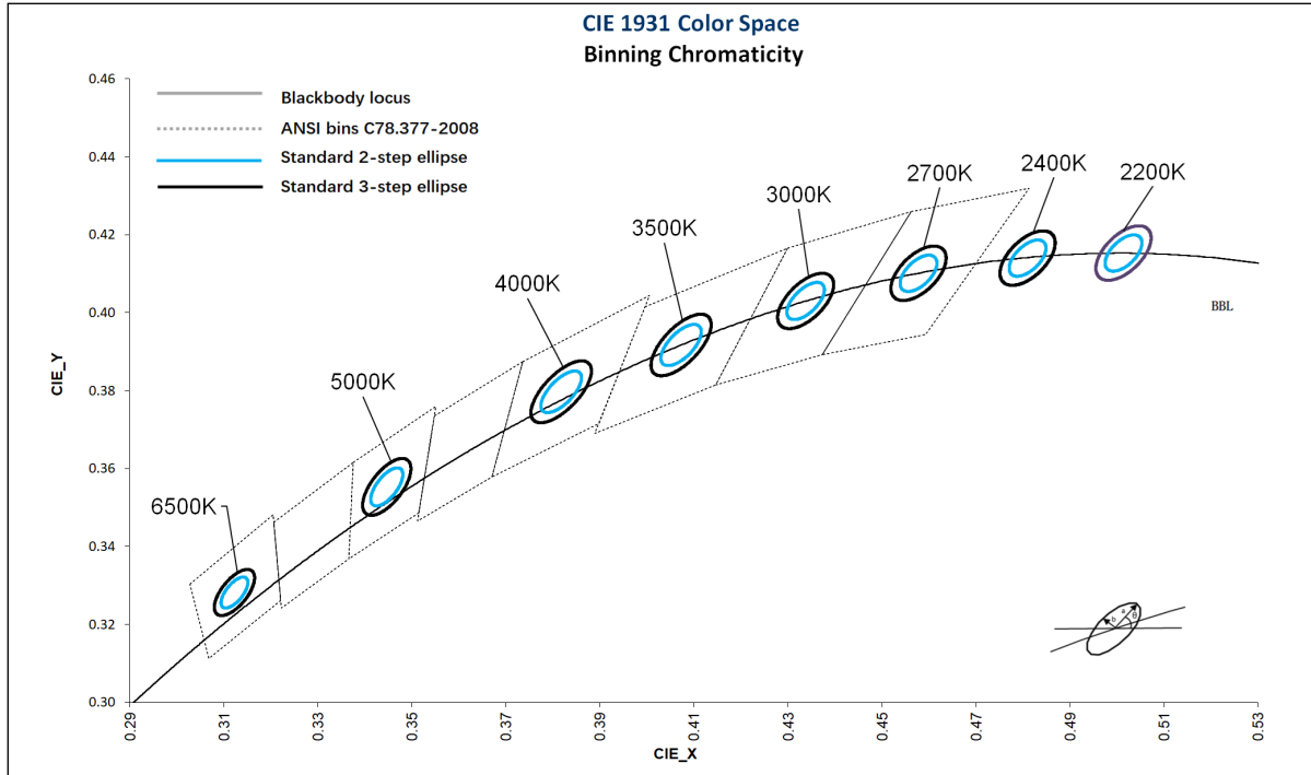
Chromaticity Binning Diagram 1 - TE60
