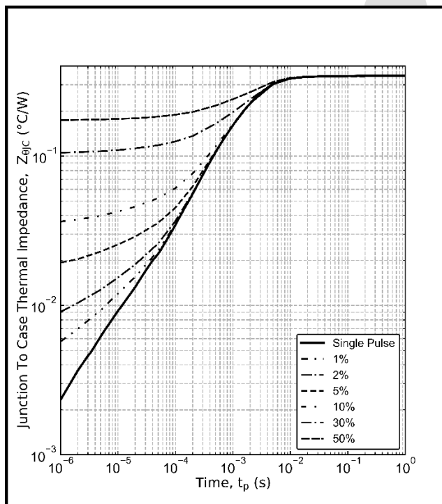
Figure 27. Transient thermal impedance
