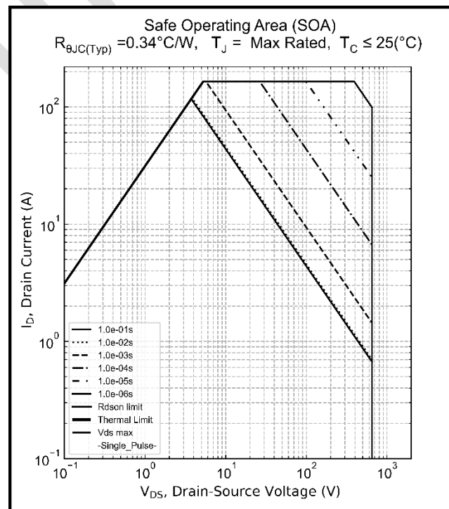
Figure 28. Safe Operating Area (SOA)
