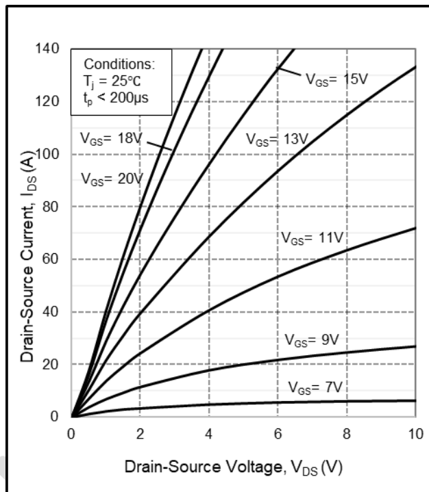
Figure 2. Output characteristics at T_j = 25^\circ\text{C}
