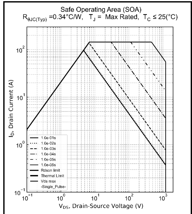
Figure 30. Safe Operating Area (SOA)
