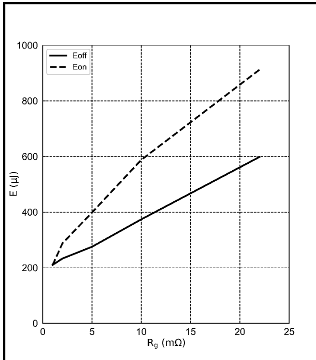
Figure 29. Typical switching energies E_{on} and E_{off} with R_g ( V_g = 0 V to 18 V , V_{ds} = 800 V , I_d = 40 A , T_j = 175^\circ C )
