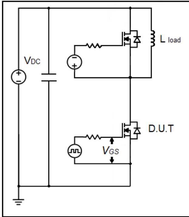
Figure 33. Clamped inductive switching waveform test circuit
