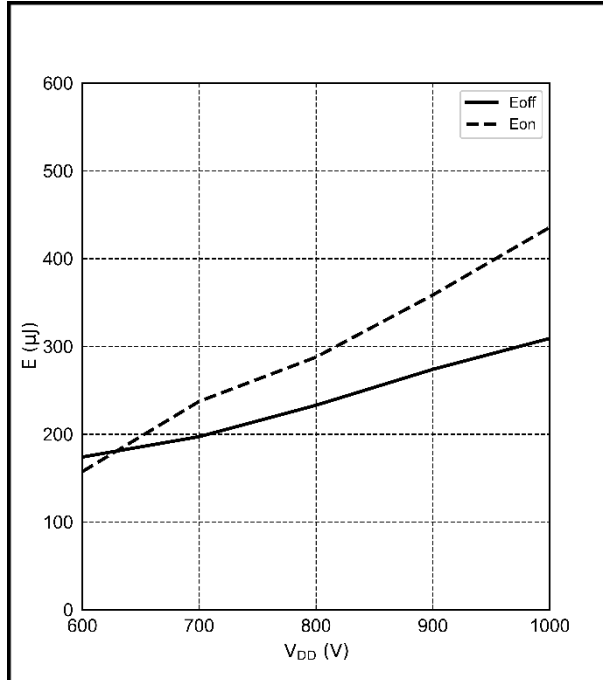
Figure 27. Typical switching energies E_{on} and E_{off} with V_{DD} ( V_g = 0 V to 18 V, I_d = 40 A, T_j = 175^\circ\text{C} , R_g = 2.2 Ω)
