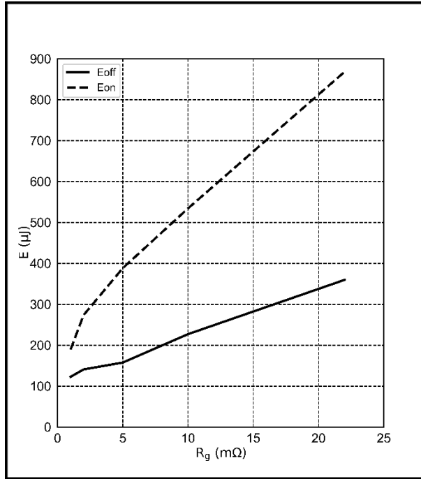
Figure 25. Typical switching energies E_{on} and E_{off} with R_g ( V_g = -5 V to 18 V, V_{ds} = 800 V, I_d = 40 A, T_j = 25^\circ\text{C} )
