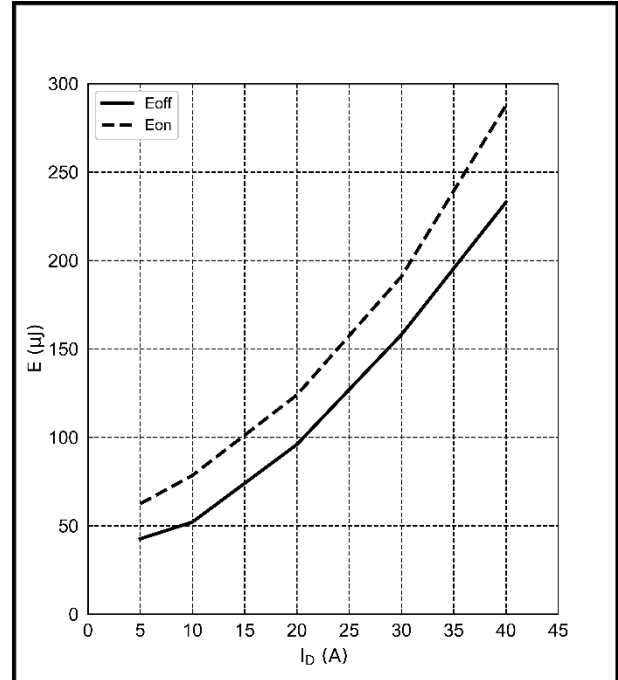
Figure 28. Typical switching energies E_{on} and E_{off} with I_D ( V_g = 0 V to 18 V, V_{dd} = 800 V, T_j = 175^\circ\text{C} , R_g = 2.2 Ω)
