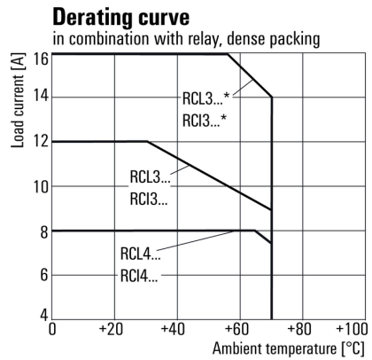
Derating curve
