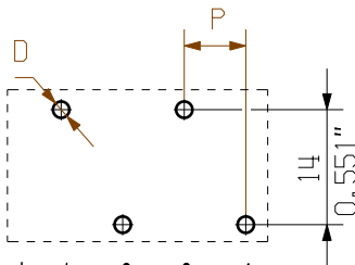
Hole pattern
